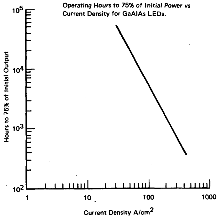
Figure 2-9. Previous Lifetime Study Results
