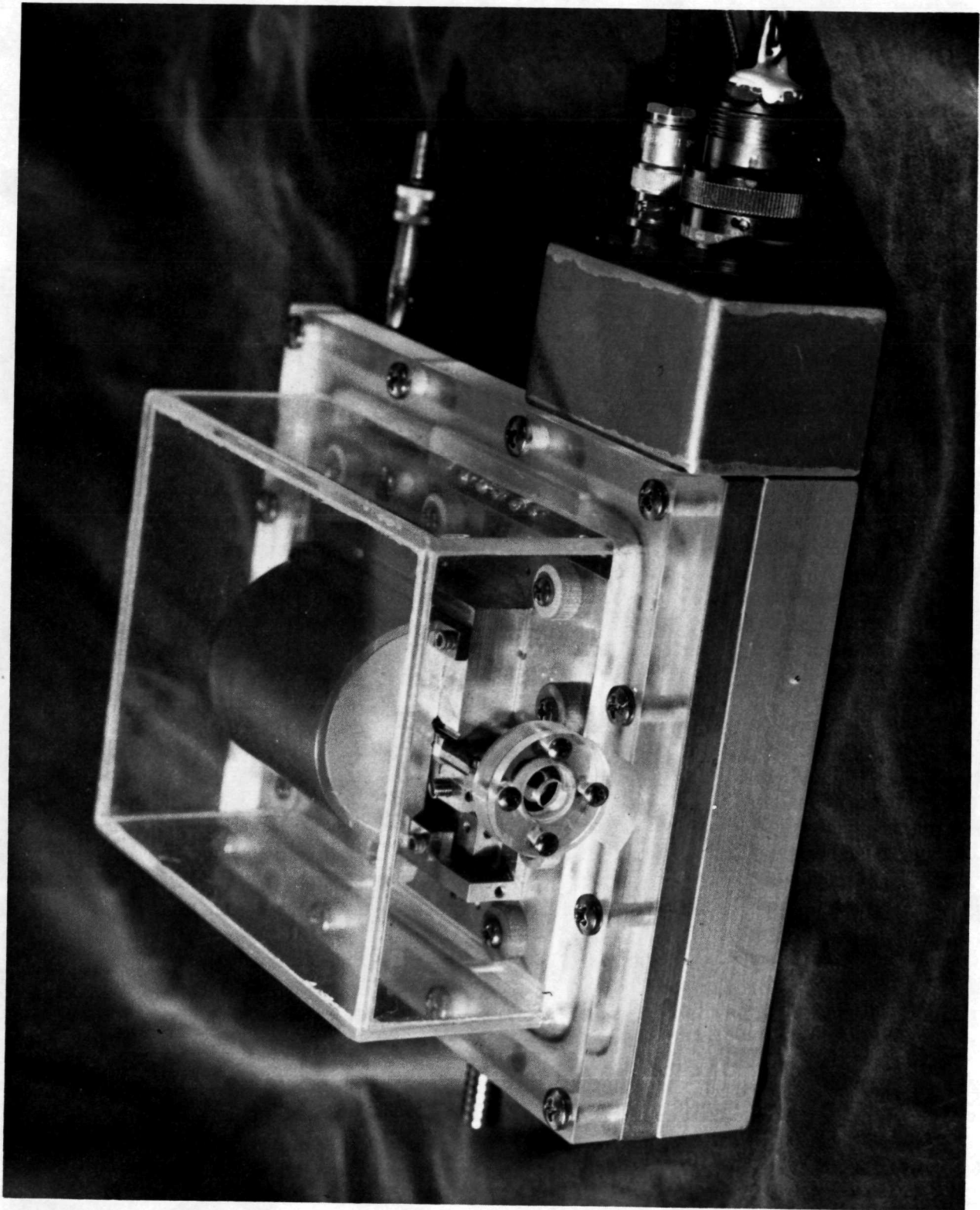
Figure 5-4. Diode Pumped Nd:YAG Device with Index Matching Solid Cylinder
