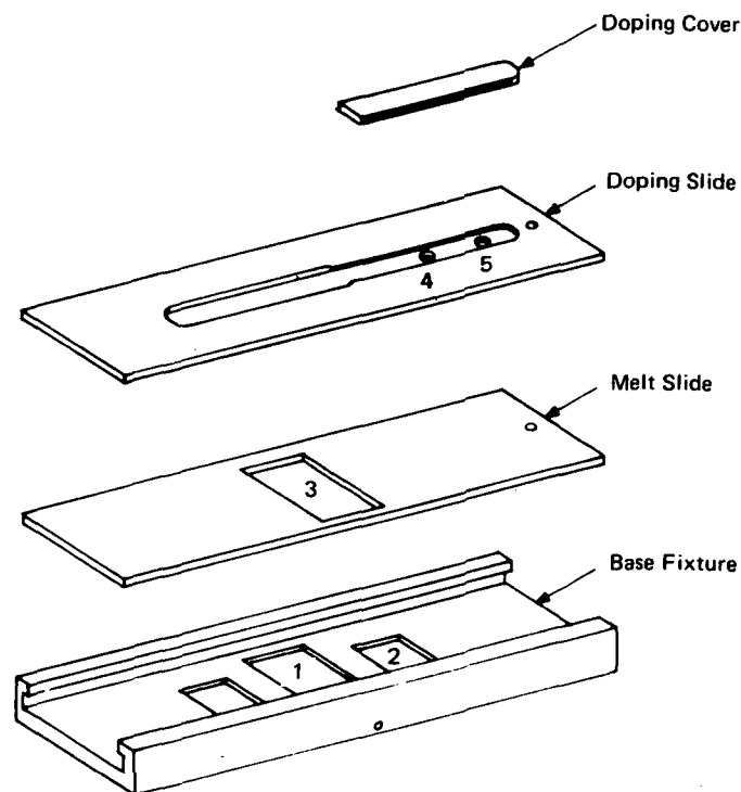
Figure 2-6. HLPE System Doping Fixture
