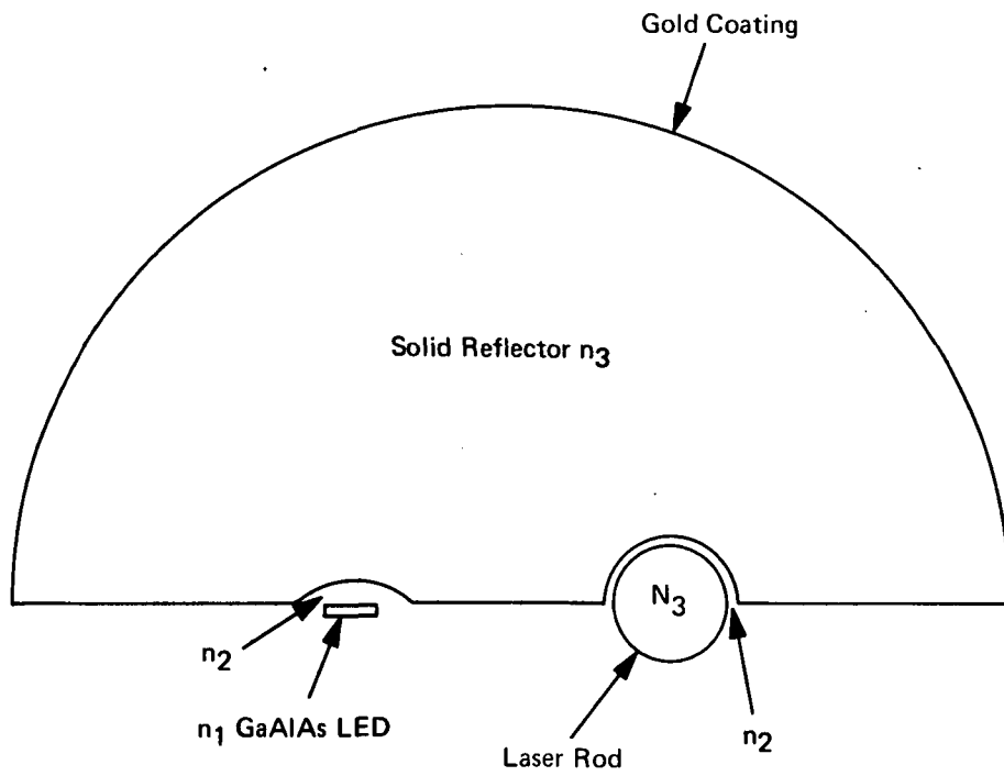
(a) Optical Index Matching
