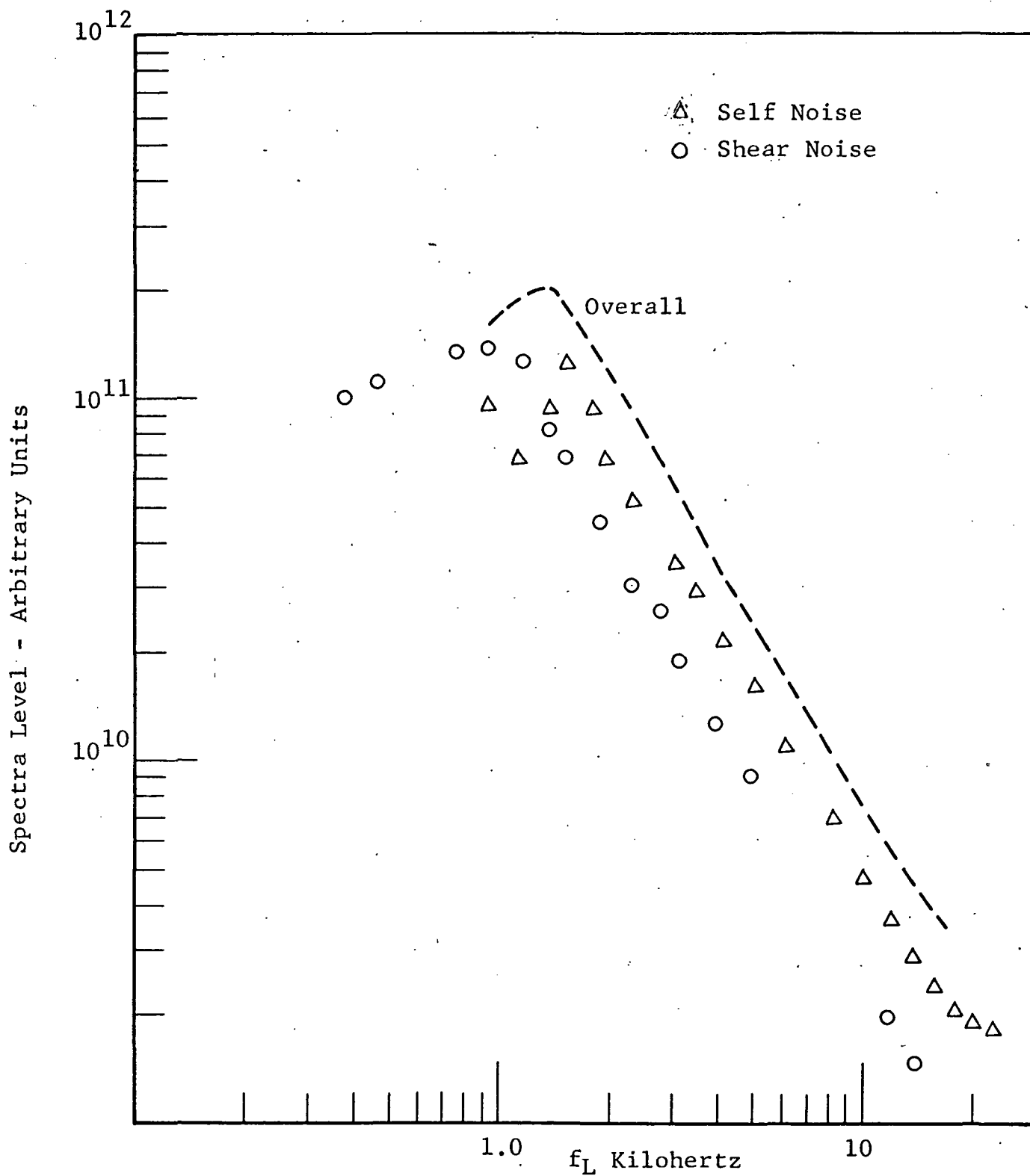
Figure 33 Jet Noise Spectrum Contributed By A Unit Volume of Turbulence At y_1/D=10.0 , r/D=0.54
