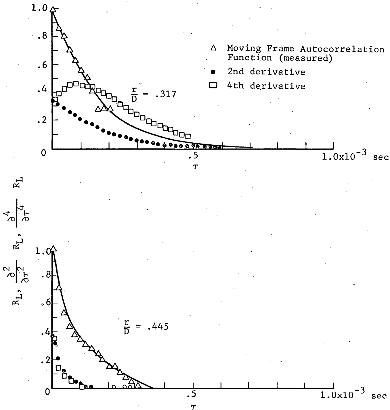
Figure 28 Moving Frame Autocorrelation And Its Derivatives \frac{y_1}{D} = 2.0 M=0.71 Jet
