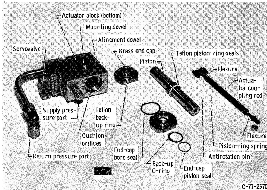
Figure 7. - Bypass valve actuator - disassembled.
