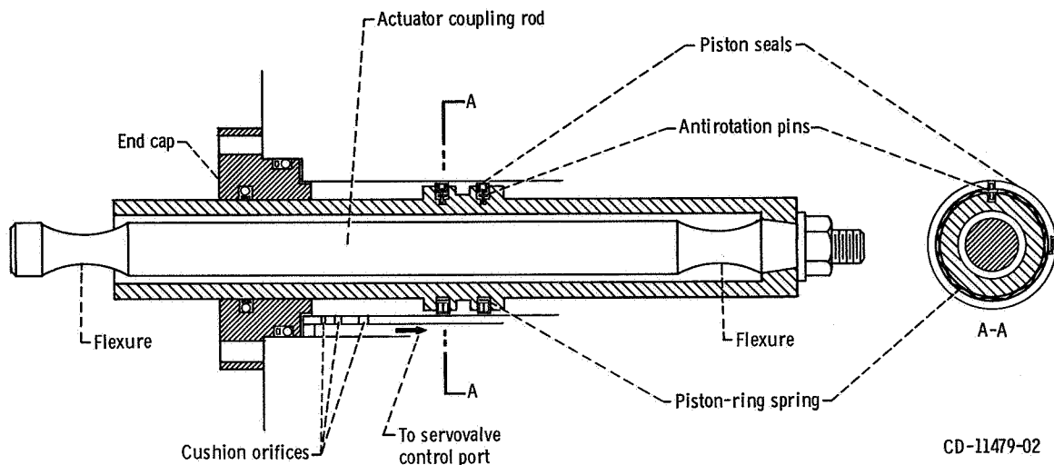
Figure 8. - Section view of assembled actuator.
