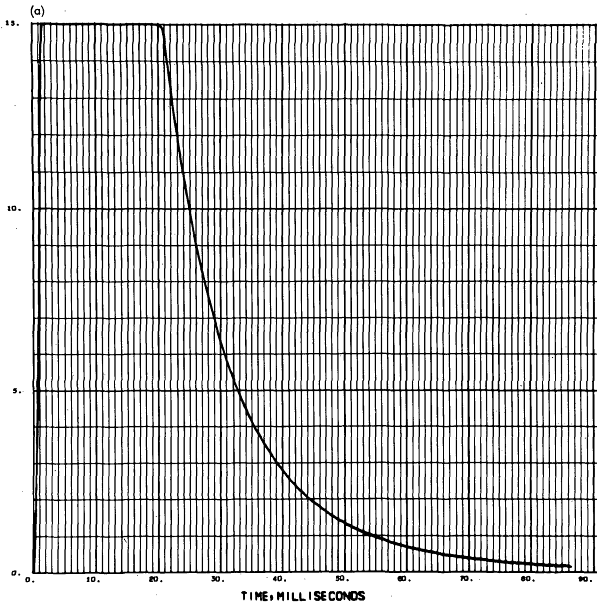
Fig. 9. MM'64 pitch/yaw valve parameters as a function of time: (a) chamber pressure, (b) total mass, nozzle, (c) total mass, chamber, (d) total mass, valve, (e) nozzle flow rate, (f) chamber flow rate, (g) valve flow rate, (h) total impulse, (i) chamber pressure derivative
