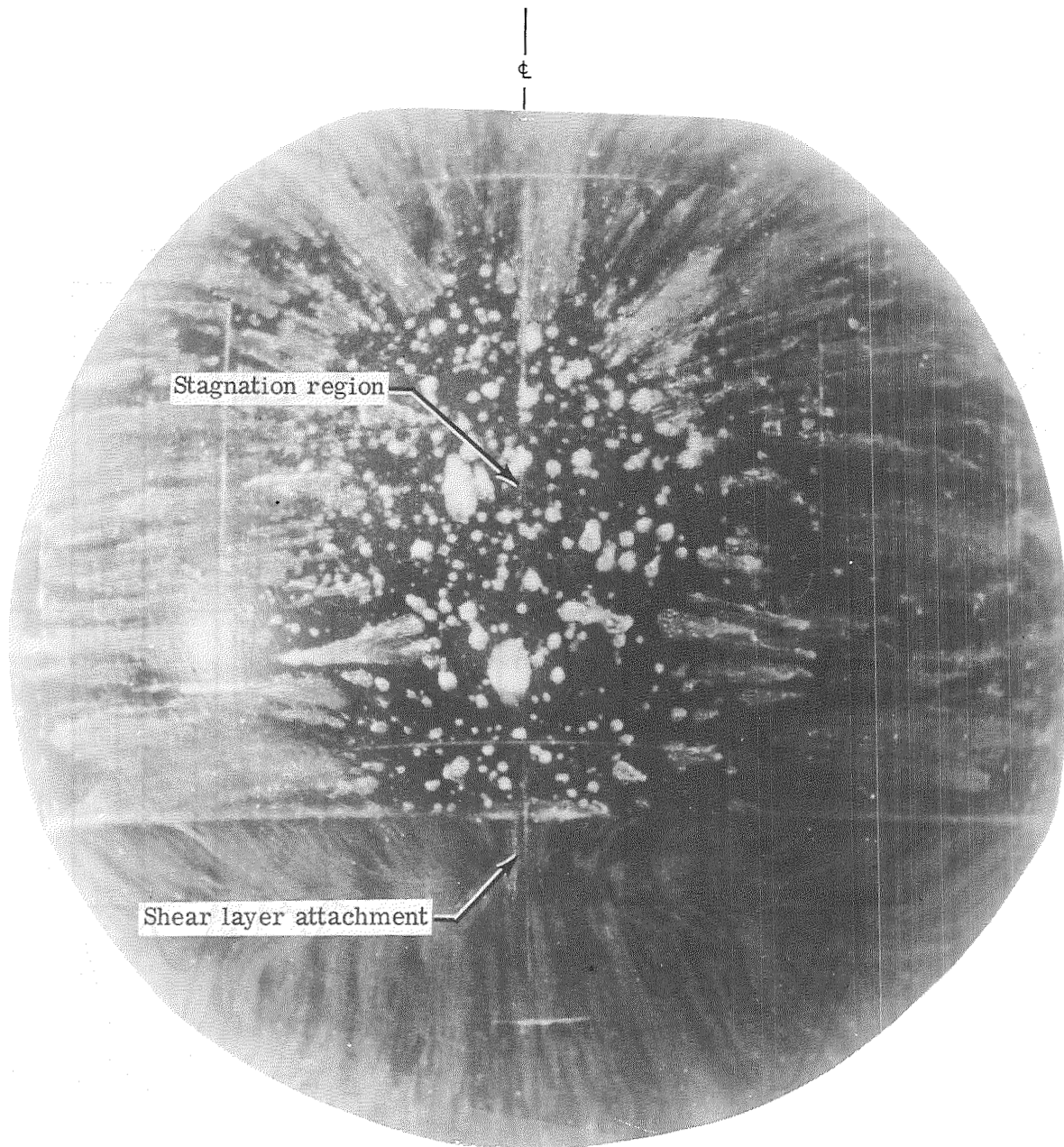
(c) Oil flow distribution.
