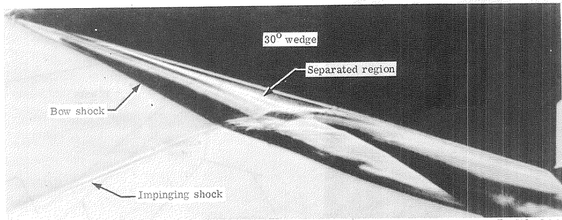
(a) Schlieren photograph.
