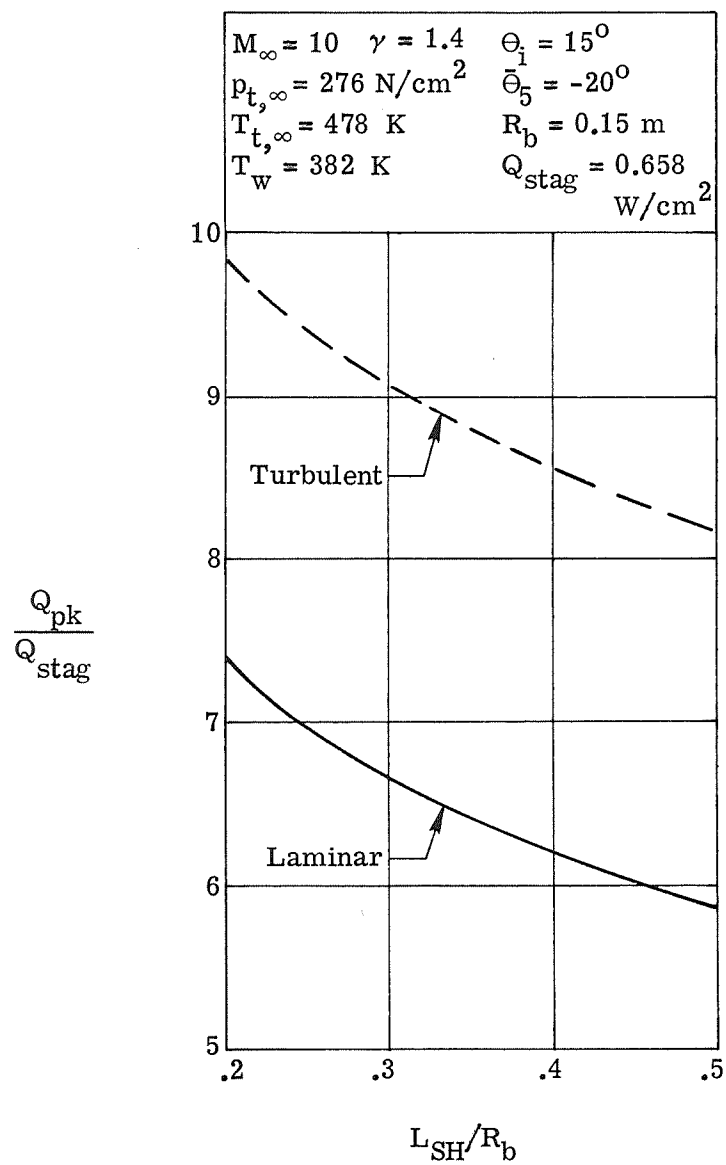
Figure 36.- Heat-transfer amplification as a function of shock displacement length (or shear layer thickness) on a 0.3-m-diameter sphere for type III interference.
