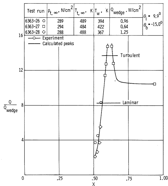
(c) Heat-transfer distribution.
