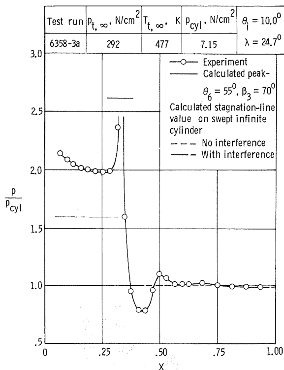
(b) Pressure distribution.
