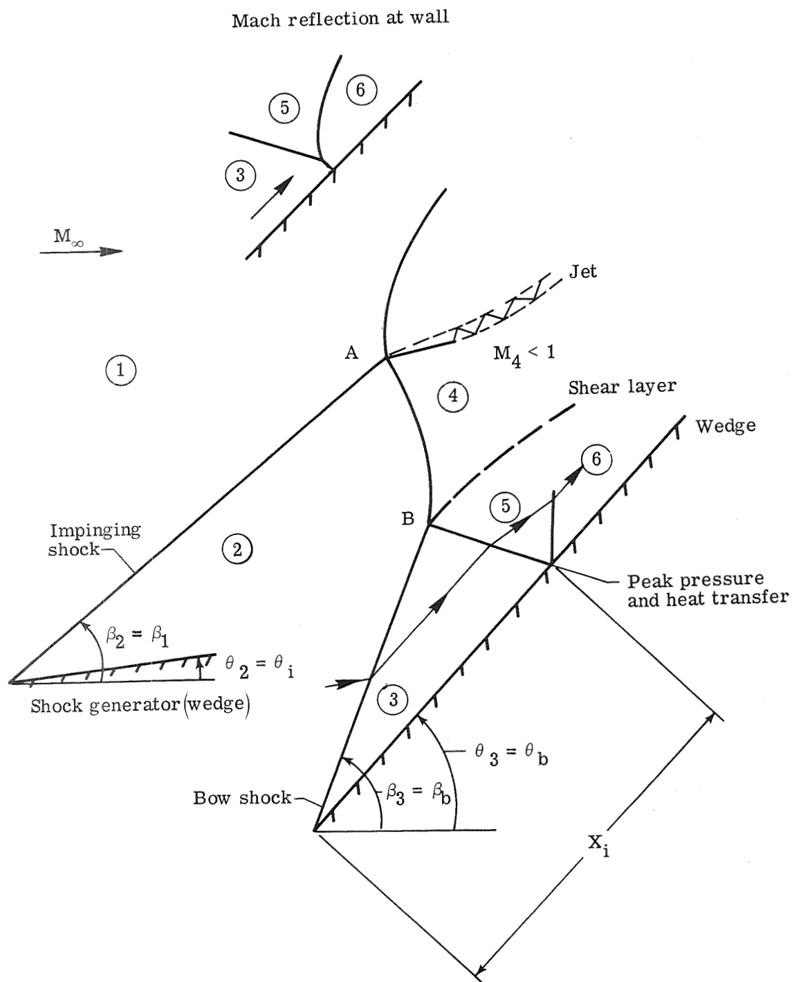
Figure 11.- Type V shock interference pattern.
