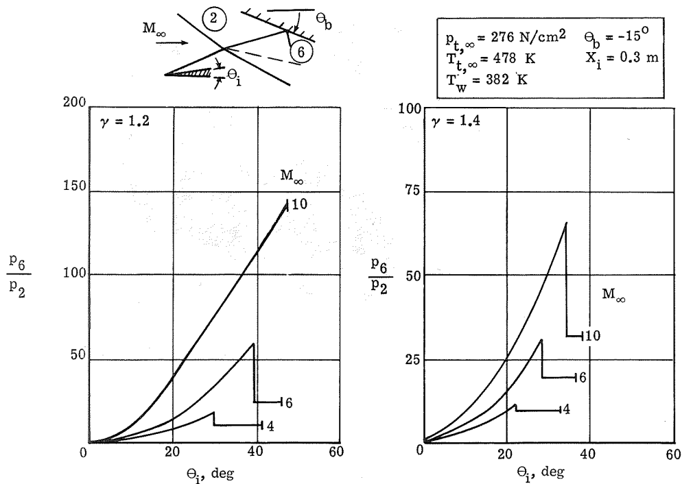
(a) Pressure amplification.
