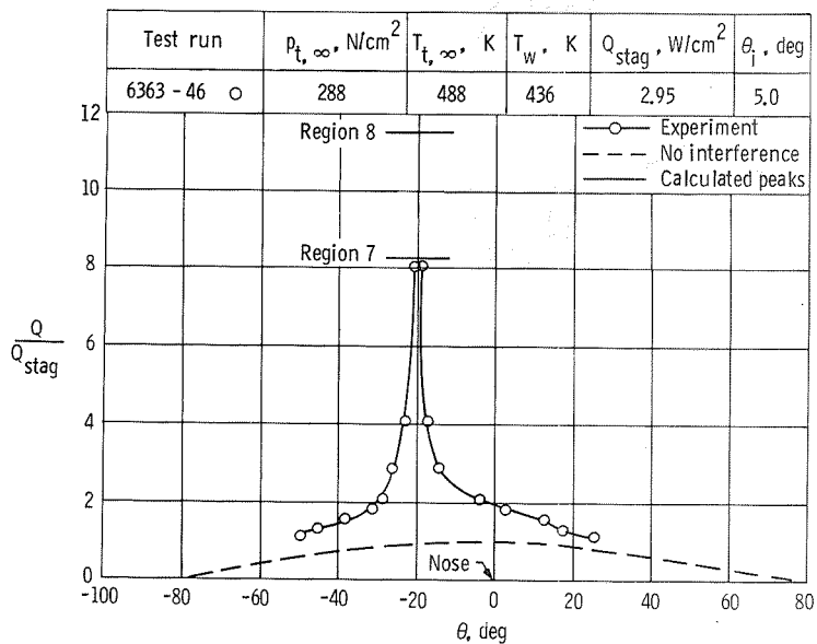
(c) Heat-transfer distribution.
