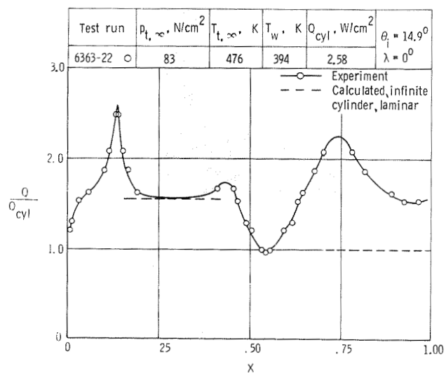
(c) Heat-transfer distribution.
