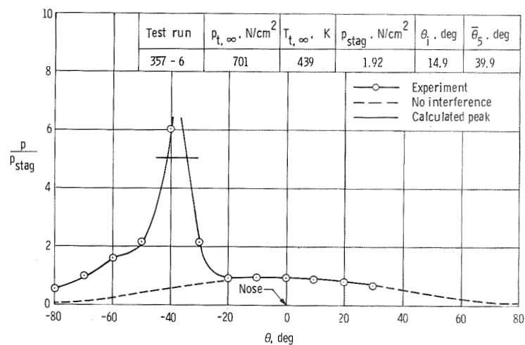
(b) Pressure distribution.
