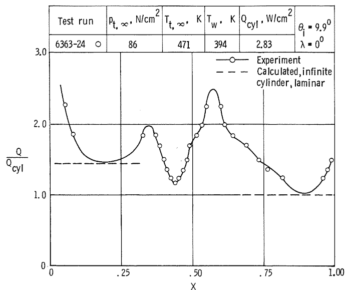
Figure 58.- Type IVa interference on a fin at Mach 5.94 in air. \theta_i \approx 10^\circ ; N_{\text{Re}, \infty}/m \approx 8.1 \times 10^6 ; \gamma = 1.4 .
