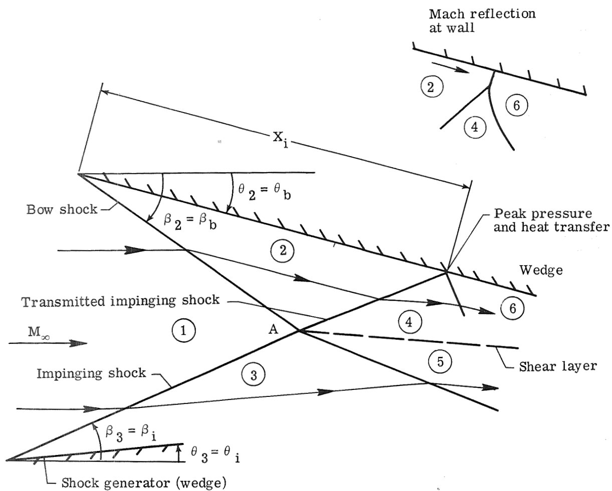
Figure 3.- Type I shock interference pattern.
