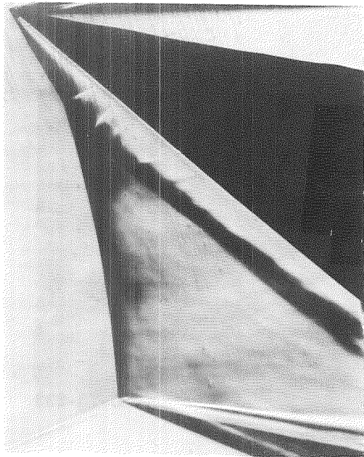
L-73-234 (a) Schlieren photograph.
