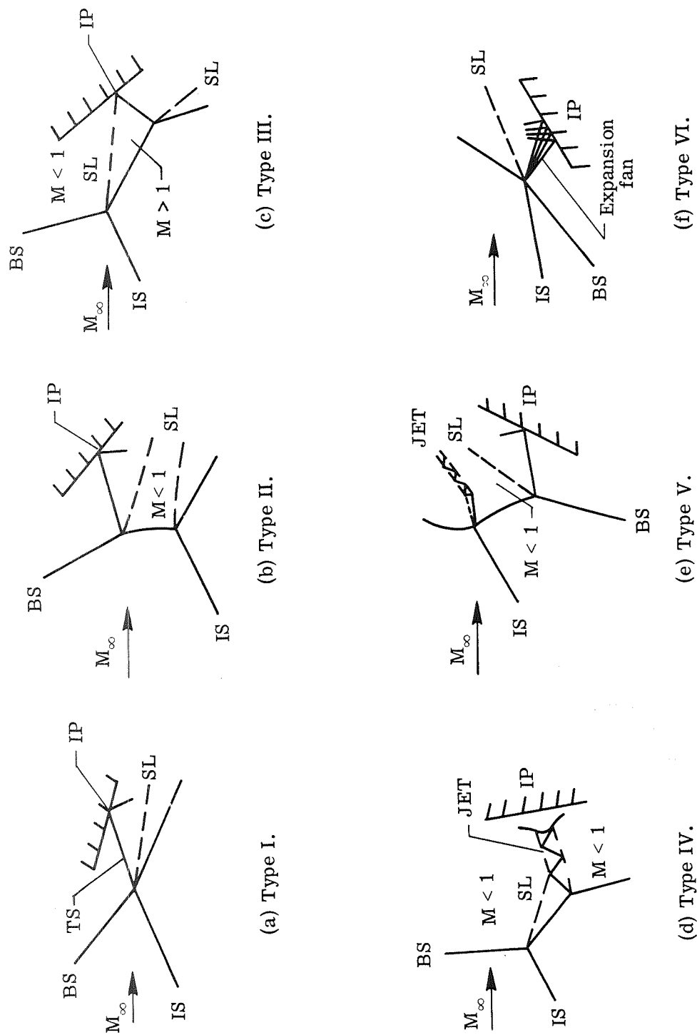
Figure 1. - Six types of shock interference patterns.
