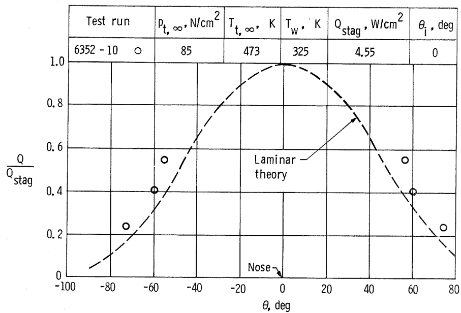
Figure 45.- Pressure and heat-transfer distribution on a 0.051-m-diameter hemisphere at Mach 5.94 in air. \theta_i = 0^\circ ; N_{Re,\infty}/m \approx 8.1 \times 10^6 ; \gamma = 1.4 .
