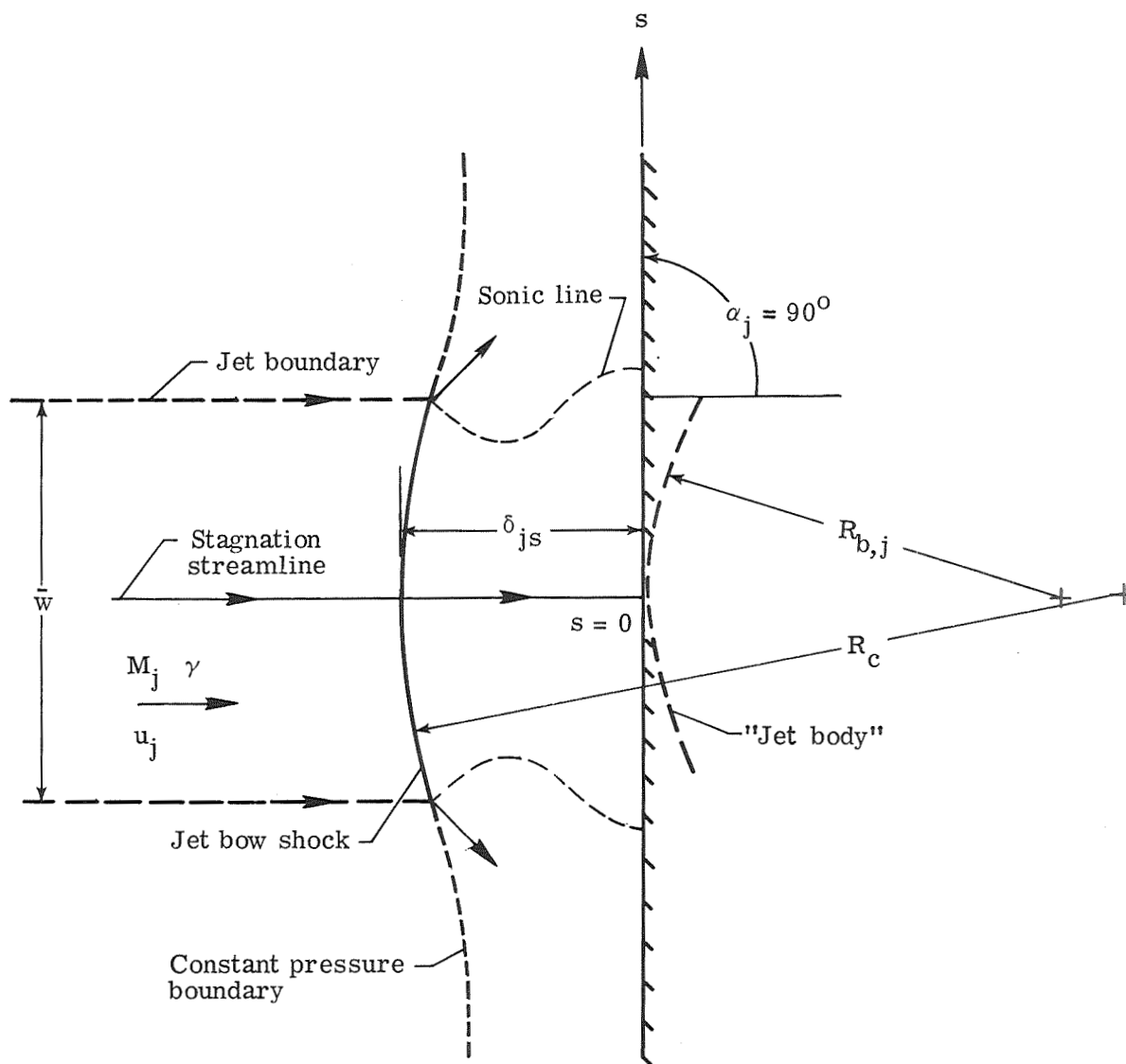
Figure 10.- Normal jet impingement model for M_j < 2.8 (ref. 57).
