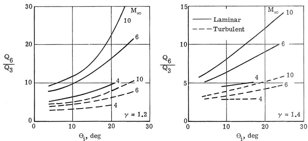
(b) Heat-transfer amplification.
