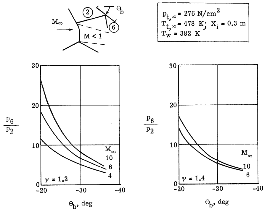
(a) Pressure amplification.
