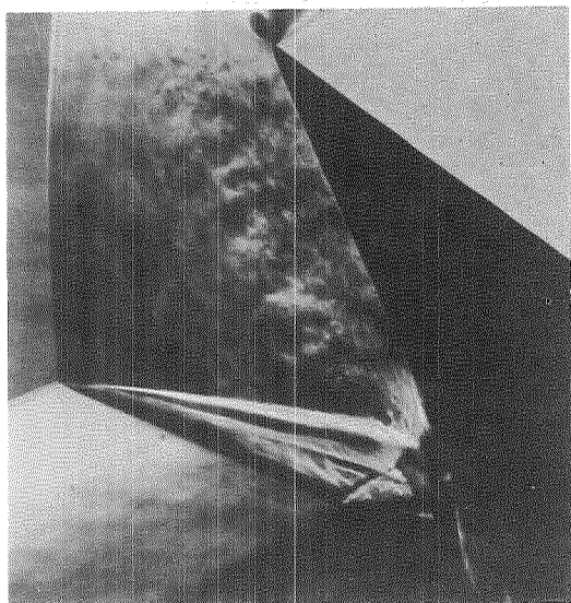
(a) Schlieren photograph.
