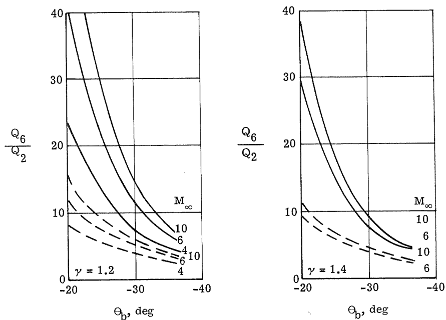
(b) Heat-transfer amplification.
