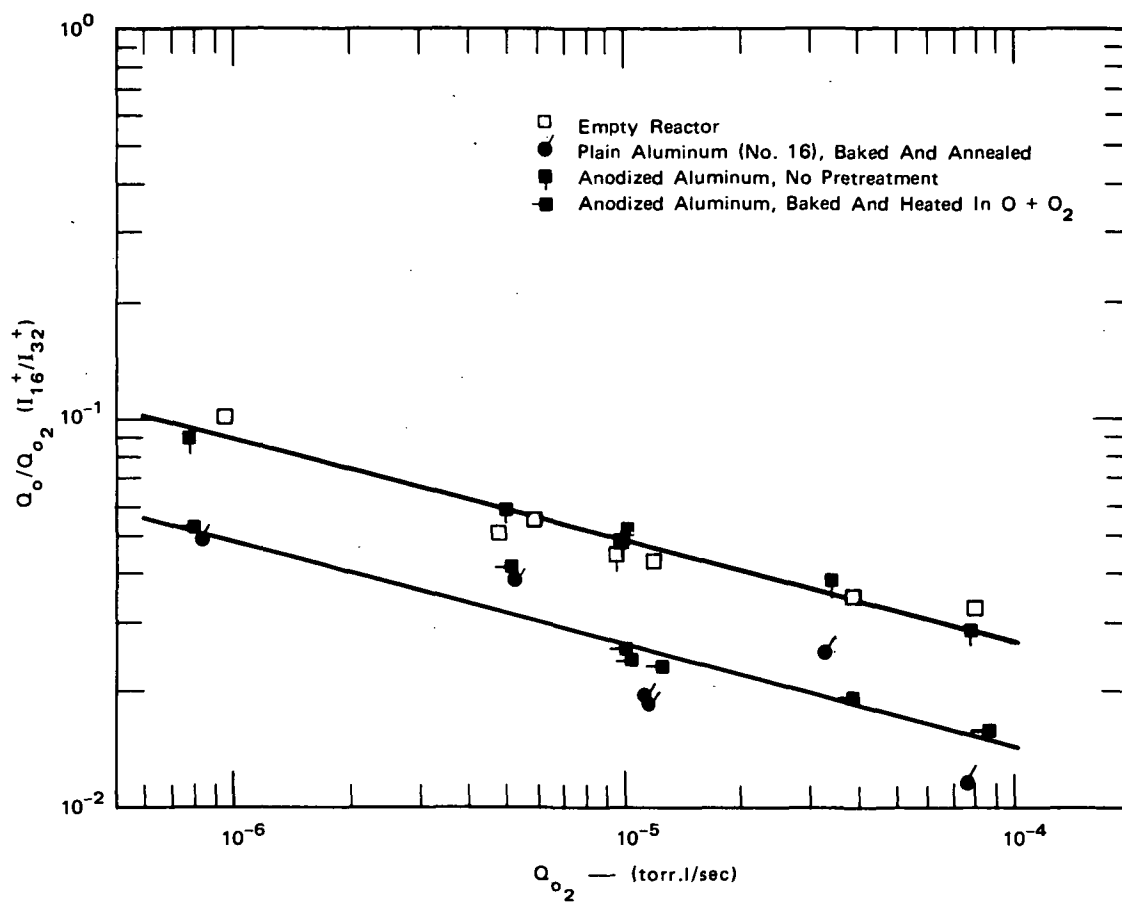
FIGURE 4 TYPICAL EXPERIMENTAL DATA. T = 330^\circ K
