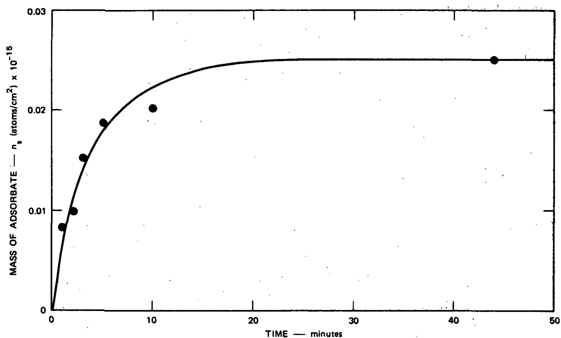
FIGURE 7 ADSORPTION OF ATOMIC OXYGEN ON PLAIN ALUMINUM (SPECIMEN NO. 6). n_g = 1.5 \times 10^9 atoms/cm 3 . T = 330^\circ\text{K} .
