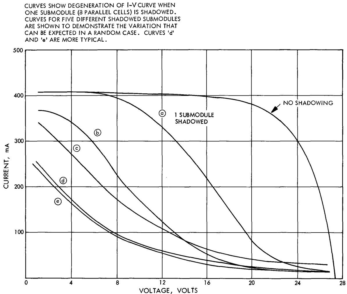
Fig. 16. Effect of Completely Shadowing Several Different Submodules (Rows of eight parallel cells)
