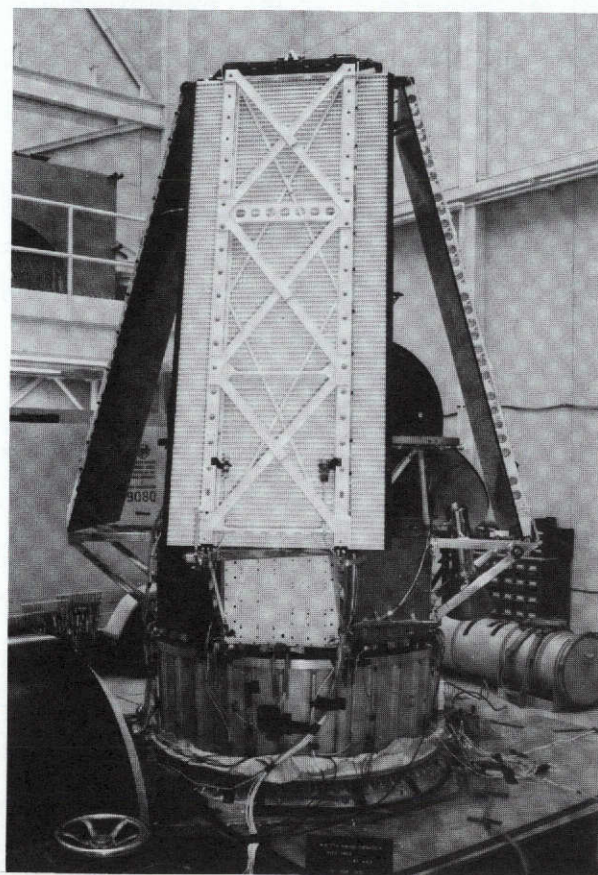
Fig. 2. Spacecraft With Solar Panels Tip-Latched
