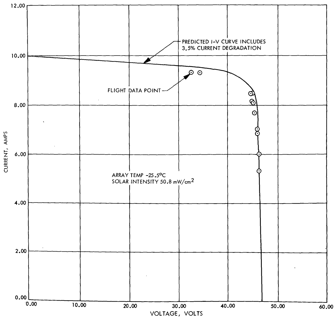
Fig. 34. Solar Array Performance During Test No. 4, October 2, 1972
