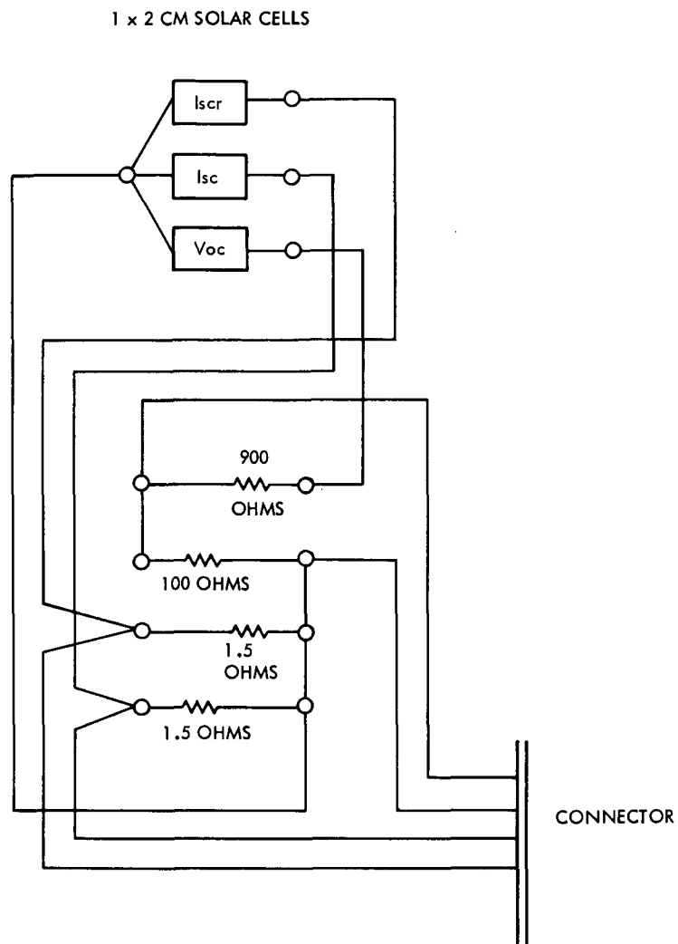
Fig. 11. Schematic Diagram of I sc -V oc Transducer
