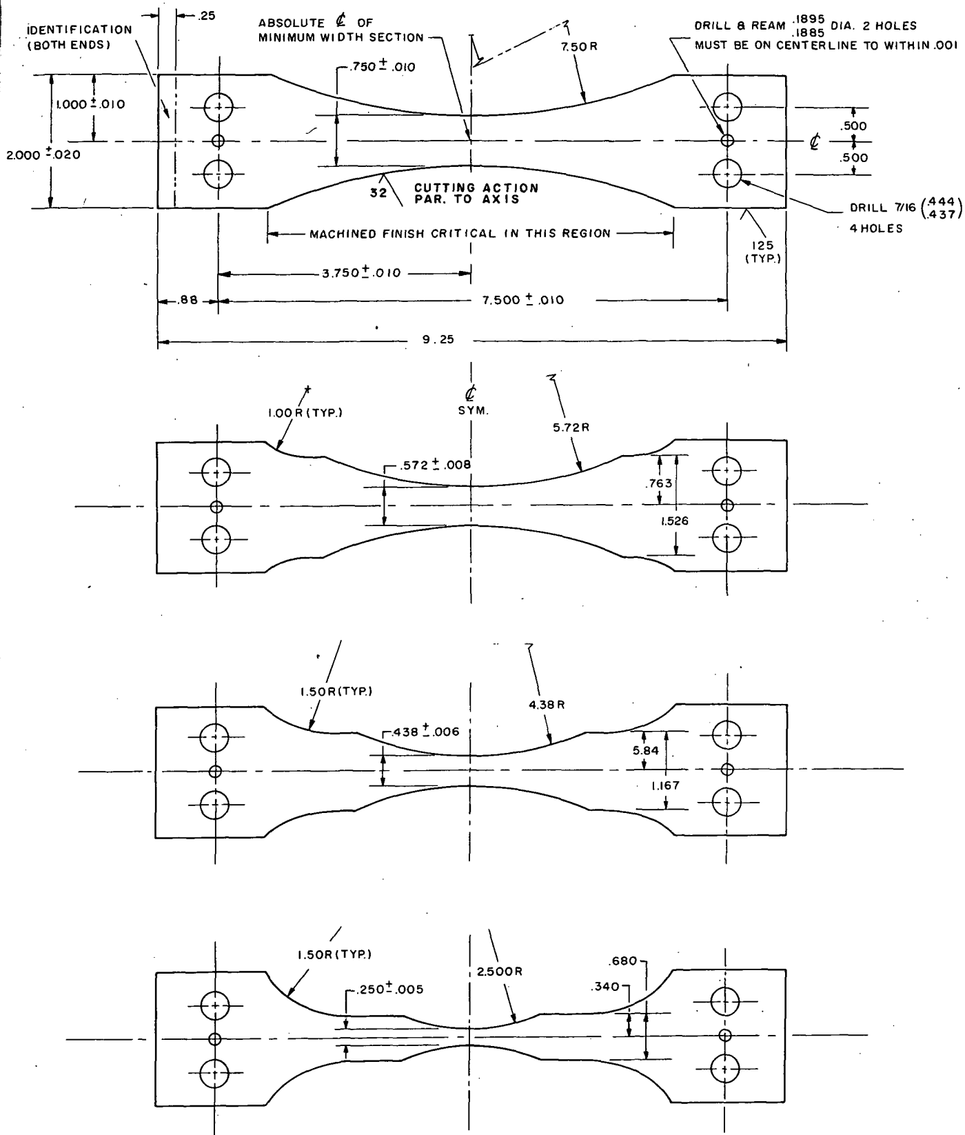
Figure 3: Fatigue Test Specimen Details
