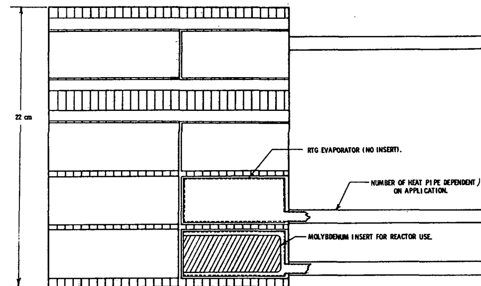
FIGURE 4. - 19 FUEL PIN CORE FOR USE AS LARGE RTG OR AS 1/2 OF A FAST REACTOR. ALL DIMENSIONS ARE THE SAME AS THOSE OF FIGURE 2 EXCEPT THE DIAMETER.
