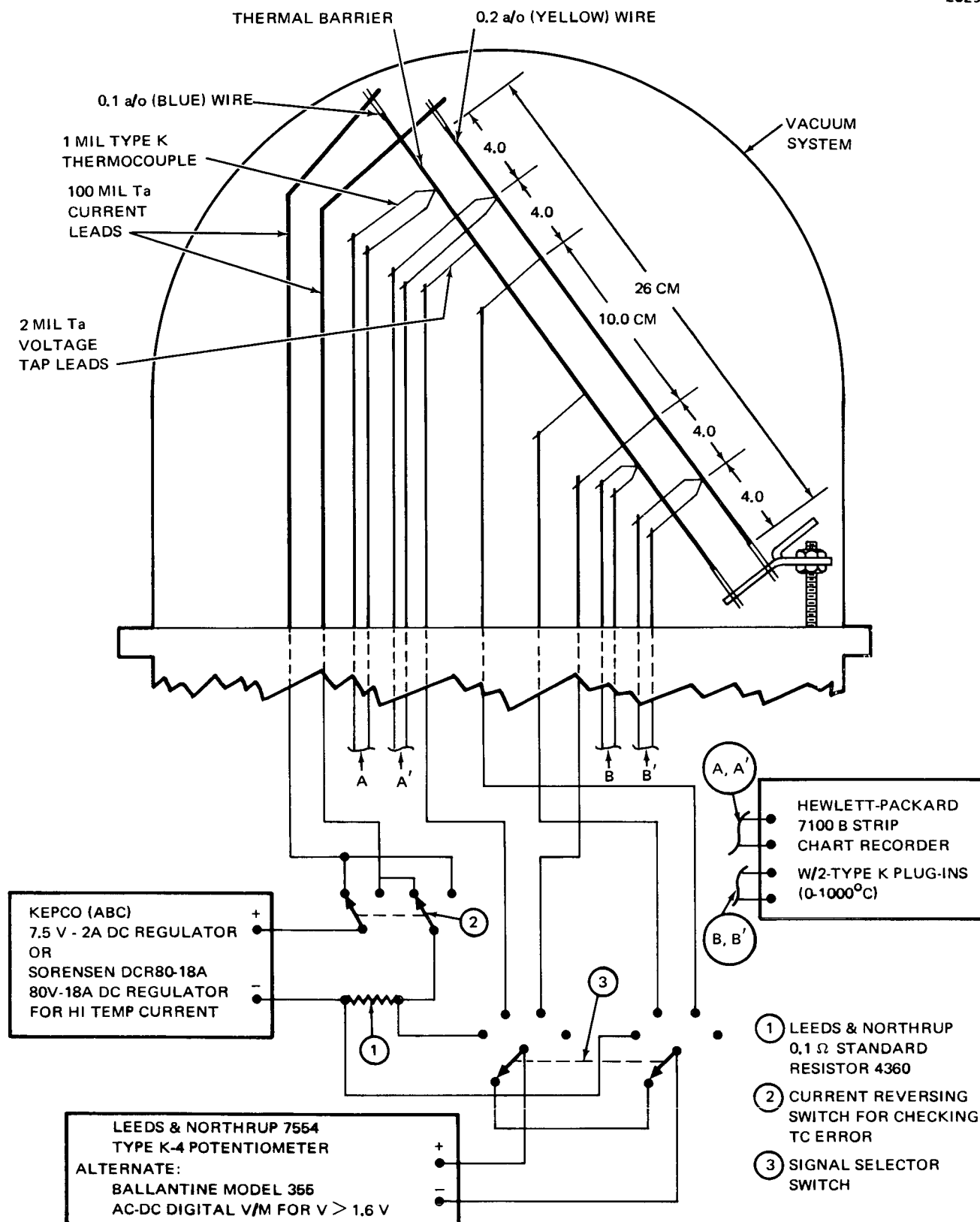
Figure 2-8. Experimental Arrangement for Temperature Calibration
