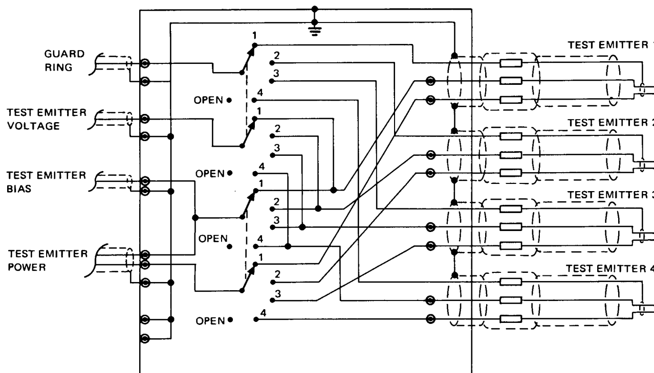
Figure 2-7. Test Emitter Selector Switch Circuit
