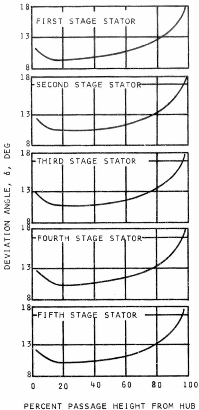
(b) Stator blade rows
