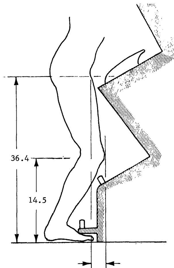
Figure VI-9 Slope & Recess Required Below Urinal Opening to Accommodate Lowering the Penile Height One Inch
