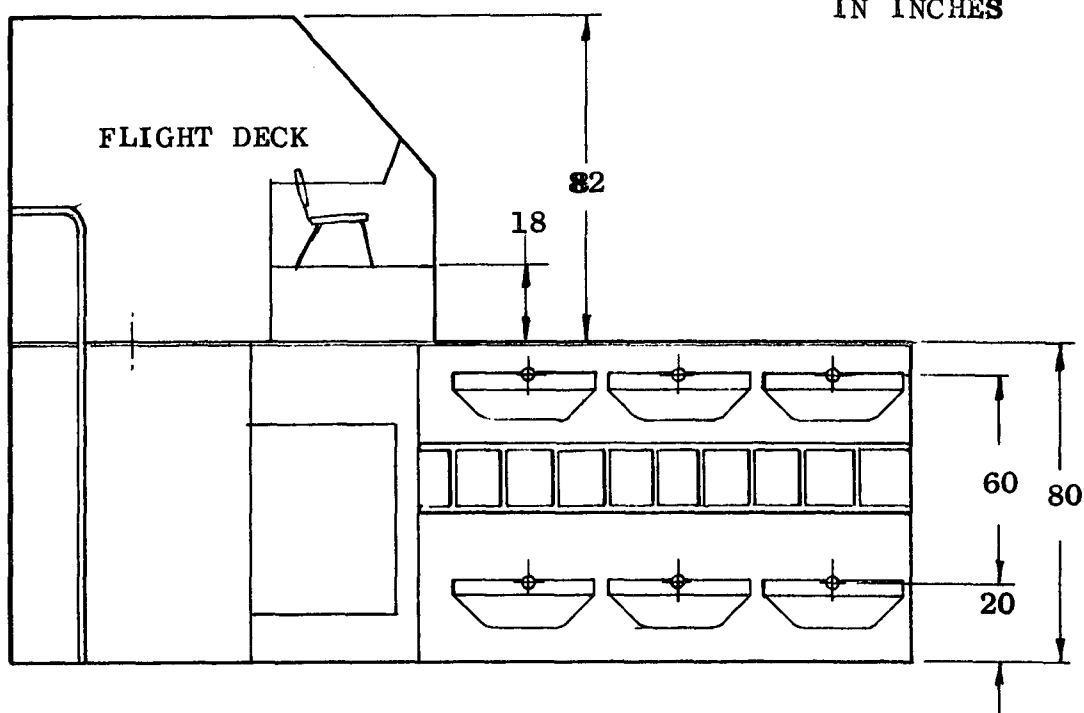
Figure III-2 Shuttle Orbiter Crew Compartment
