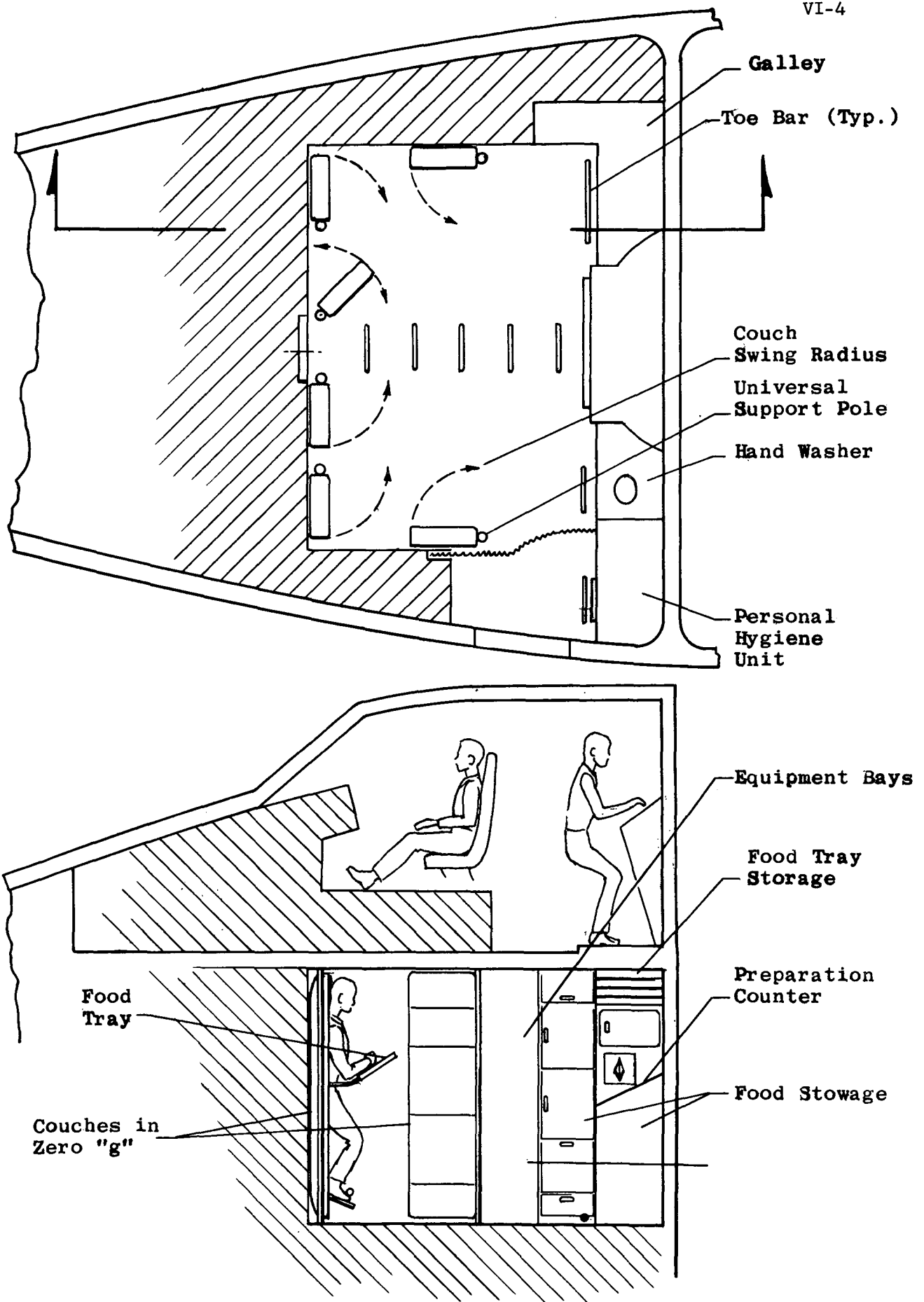
Figure VI-2 Shuttle Crew Compartment Layout - Zero Gravity
