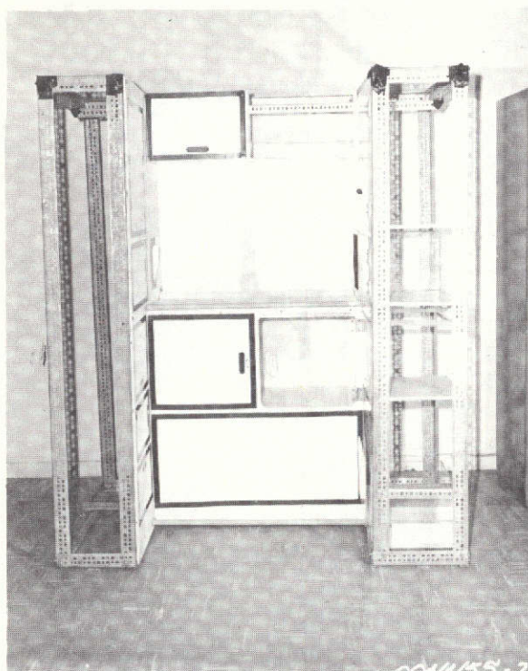
Figure IV-5 Shuttle Galley Modular Mockup
