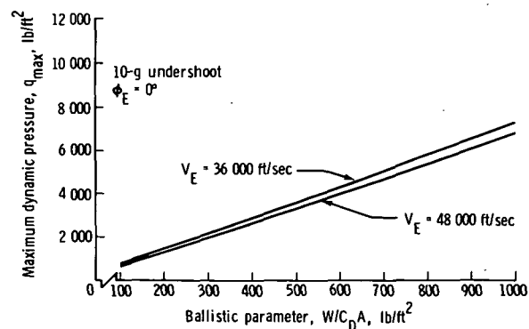
(c) L/D = 1.00 .
