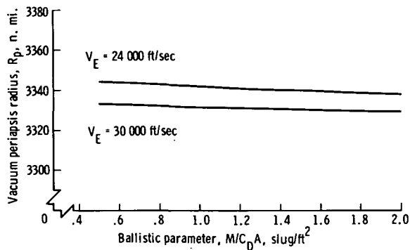
(a) L/D = 0 .
