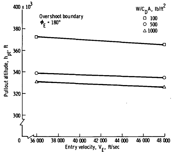
(c) L/D = 1.00 .
