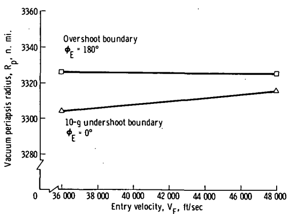
(e) L/D = 0.50 , W/C_D A = 500 \text{ lb/ft}^2 .
