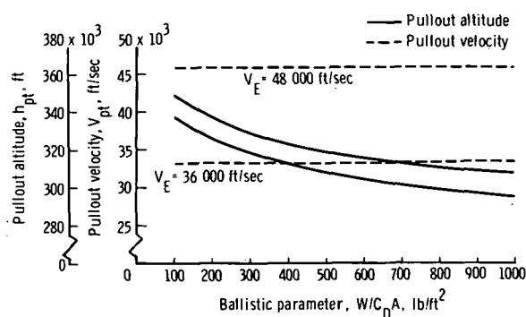
(c) L/D = 1.00 .
