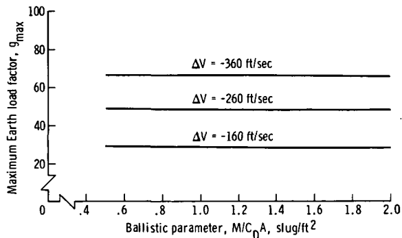
Figure 33.- Maximum Earth load factor as a function of spacecraft ballistic parameter for entry from a 200- by 10 000-n. mi. elliptical orbit; L/D = 0 .
