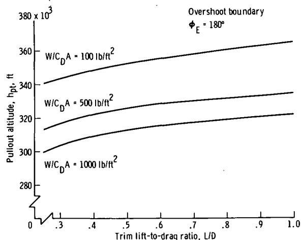
(b) V_E = 48\,000 ft/sec.
