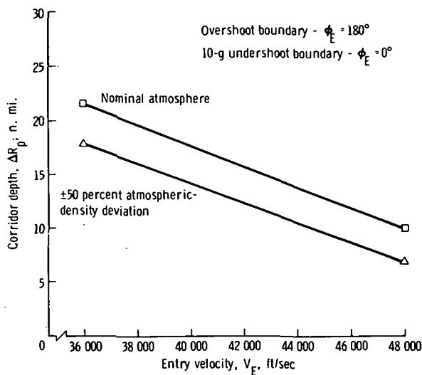
(a) L/D = 0.50 .
