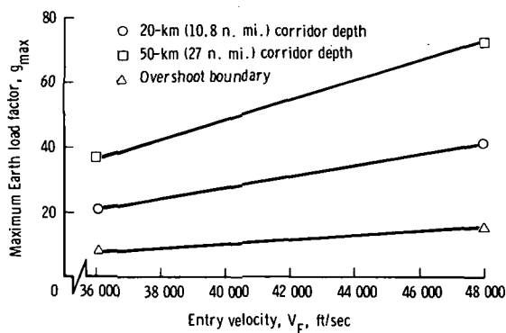
(c) L/D = 0, M/C_D A = 1.0 \text{ slug/ft}^2 .
