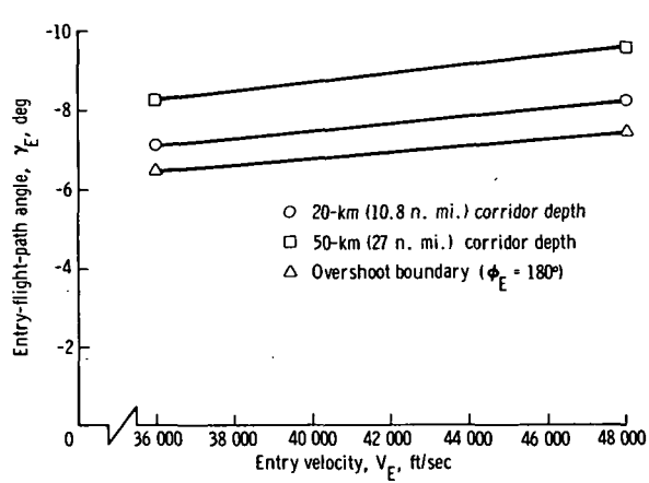
(h) L/D = 0.25 , M/C_D A = 2.0 \text{ slug/ft}^2 .
