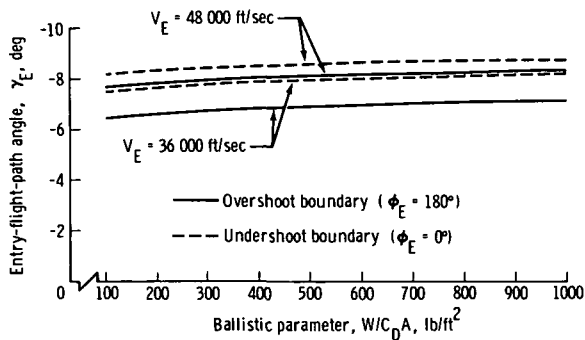
(a) L/D = 0.25.
