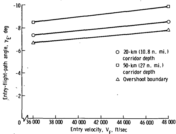
(c) L/D = 0 , M/C_D A = 1.0 \text{ slug/ft}^2 .
