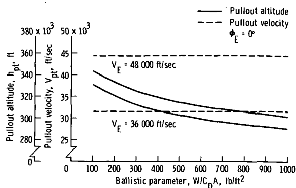
(b) L/D = 0.50 .
