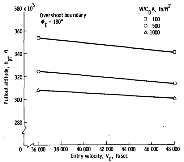
(a) L/D = 0.25 .
