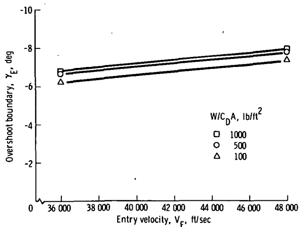
(c) L/D = 1.00 .
