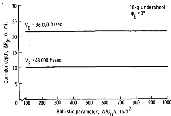
(b) L/D = 0.50 .
