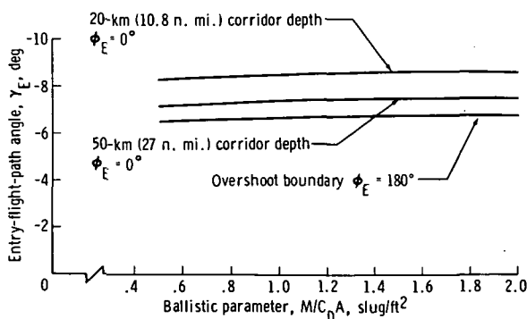
(a) L/D = 0 , V_E = 36\,000 ft/sec.
