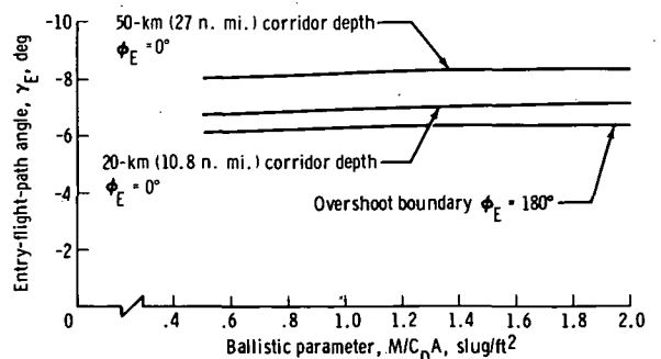
(b) L/D = 0.25 , V_E = 36\,000 ft/sec.
