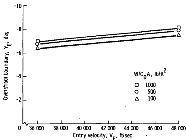
(b) L/D = 0.50 .
