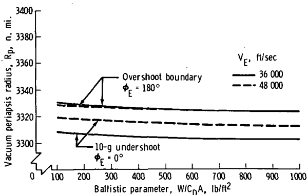
(b) L/D = 0.50 .
