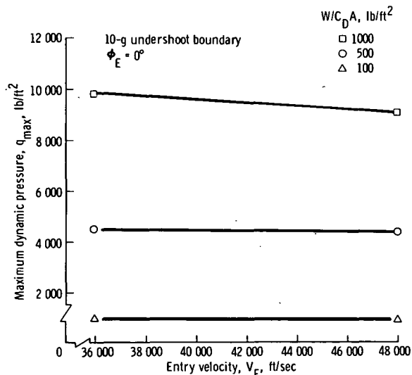
(b) L/D = 0.50 .
