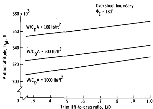
(a) V_E = 36\,000 ft/sec.
