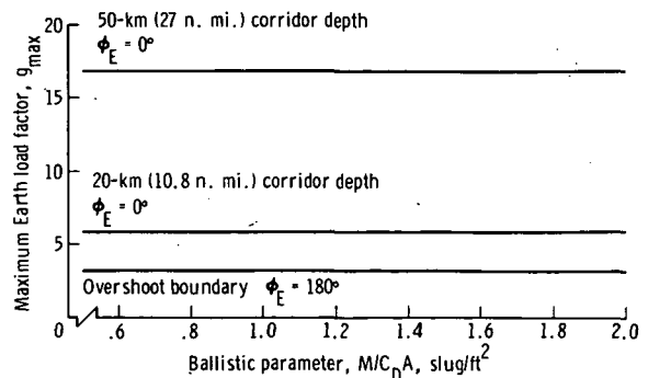
(b) L/D = 0.25 , V_E = 36\,000 ft/sec.
