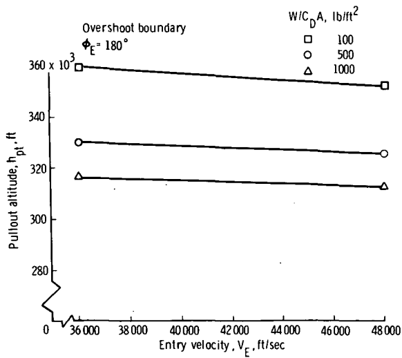
(b) L/D = 0.50 .
