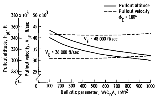
(a) L/D = 0.25 .
