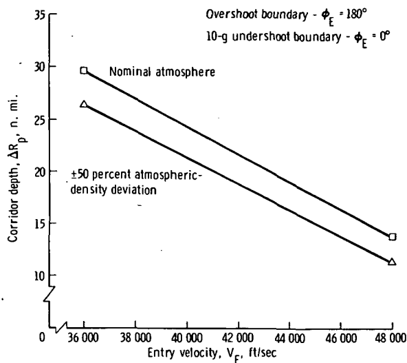
(b) L/D = 1.00 .
