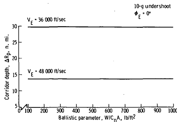
(c) L/D = 1.00 .
