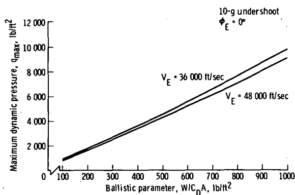
(b) L/D = 0.50 .
