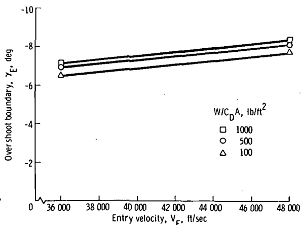
Figure 11. - Overshoot boundary entry-flight-path angle as a function of entry velocity.
