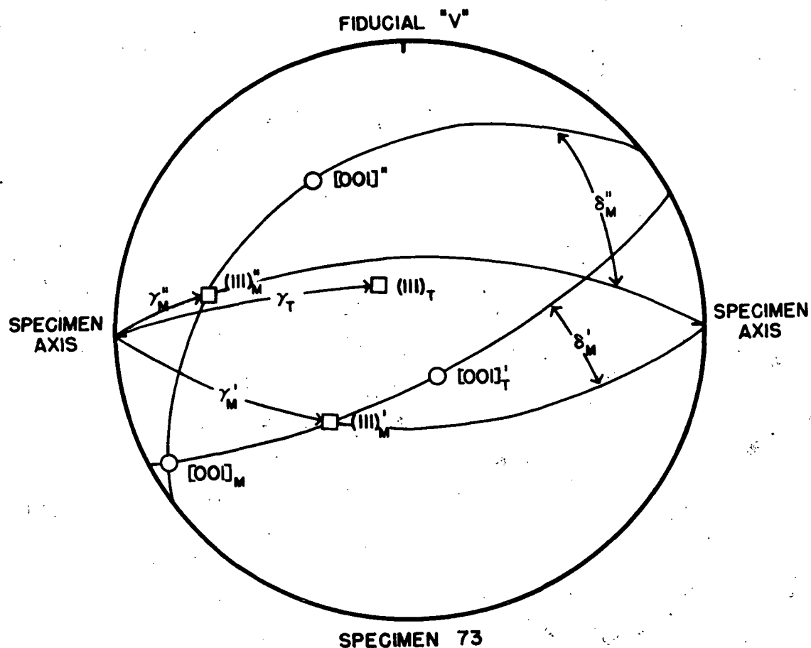
Figure 19. Stereographic projection of single region Specimen 73. The subscript "T" refers to the transformation twin system orientation and "M" to the mechanical twin system. The former cannot operate because \gamma_T \approx \pi/2 (Section III, Expression 1). Both transformation twins, [001]_T' and [001]_T'' , are twin related to a mechanical twin, [001]_M , across the (111)_M' and (111)_M'' twin planes respectively. Owing to favorable \gamma and \delta (not shown) values, the [001]_M is favorably oriented to relieve compressive stress.
