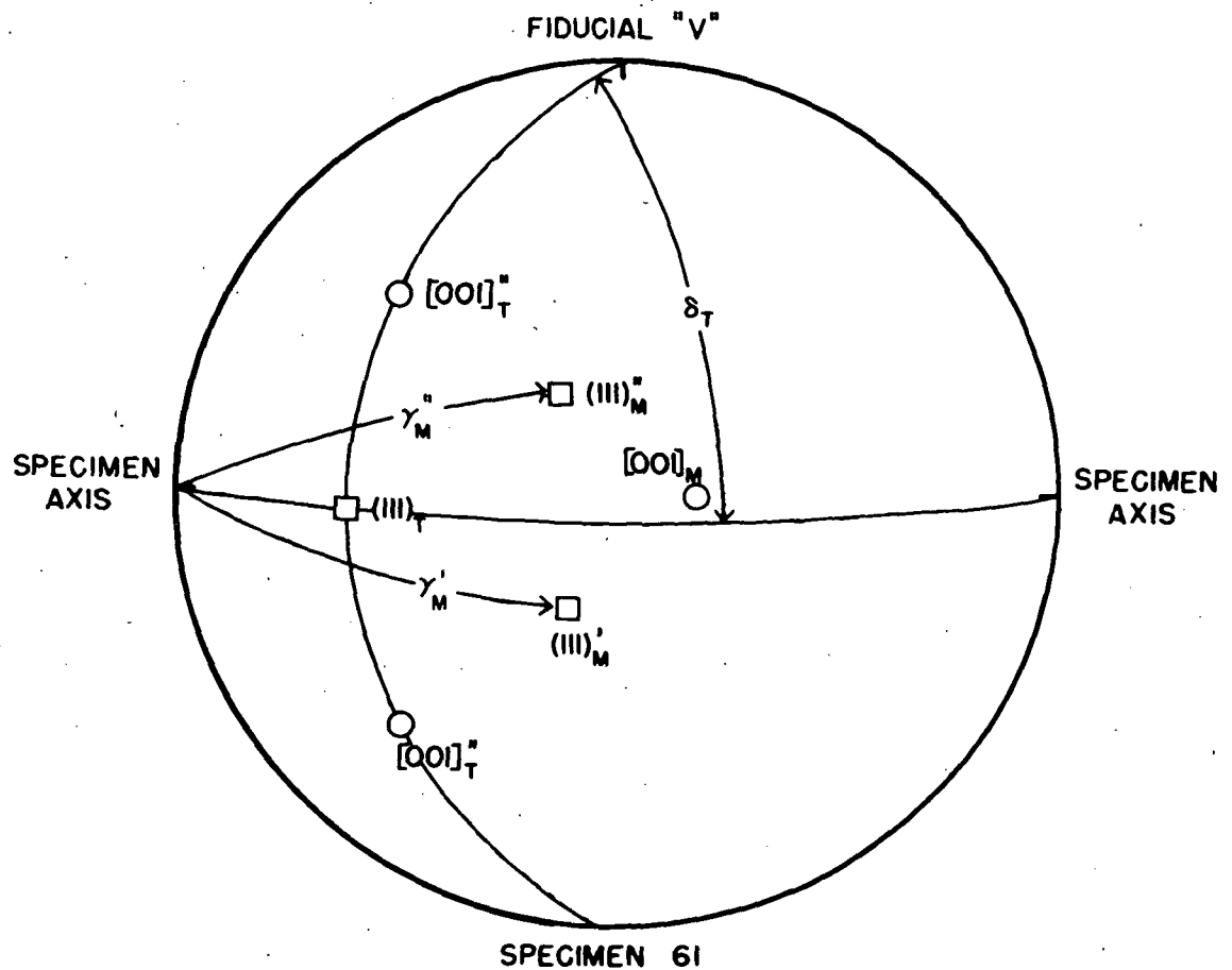
Figure 24. Stereographic projection of Specimen 61. The subscript "T" refers to the transformation twin system which cannot operate because \delta_T \approx \pi/2 (Section III, Expression 1). Likewise, mechanical twinning cannot occur because \gamma_M' and \gamma_M'' \approx \pi/2 for each mechanical twin plane in the above mentioned expression.
