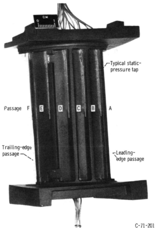
(b) Before porous shell was welded to strut - suction side.
