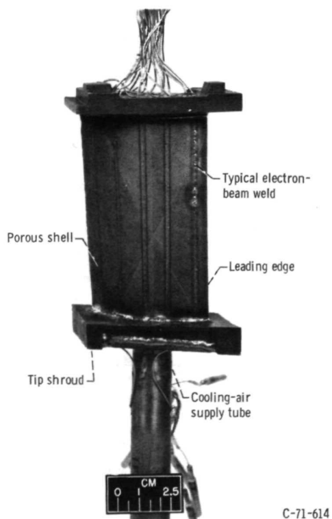
(c) After porous shell was welded to strut.
