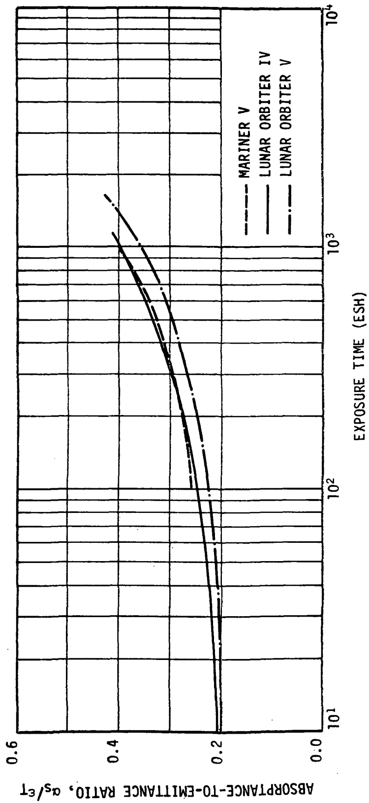
ANALYZED ABSORPTANCE-TO-EMISSION RATIO OF S-13G
