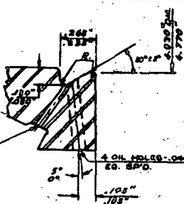
LARGE END RIB DETAIL
