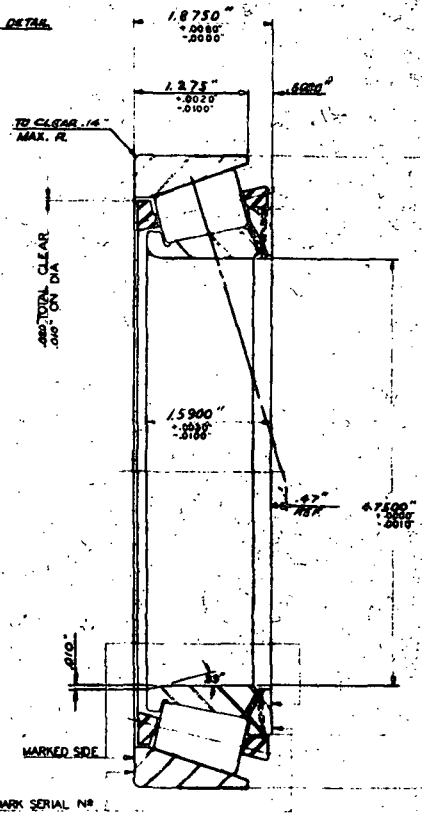
LARGE END RIB DETAIL
