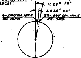
HOLE RELATIONSHIPS
