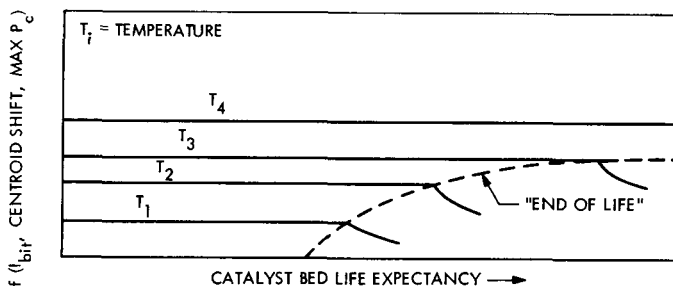
(b) ANTICIPATED INCREASE IN CATALYST BED LIFE EXPECTANCY AS A FUNCTION OF THRUSTER INITIAL TEMPERATURE (HEATED THRUSTER)
