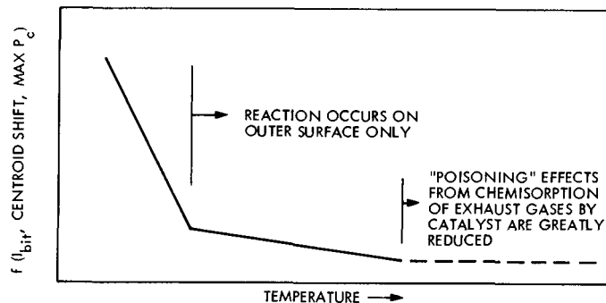
(a) ANTICIPATED EFFECTS WHEN HYDRAZINE DECOMPOSITION REACTION OCCURS ONLY ON OUTER SURFACE OF CATALYST AND WHEN CHEMISORPTION IS GREATLY REDUCED
