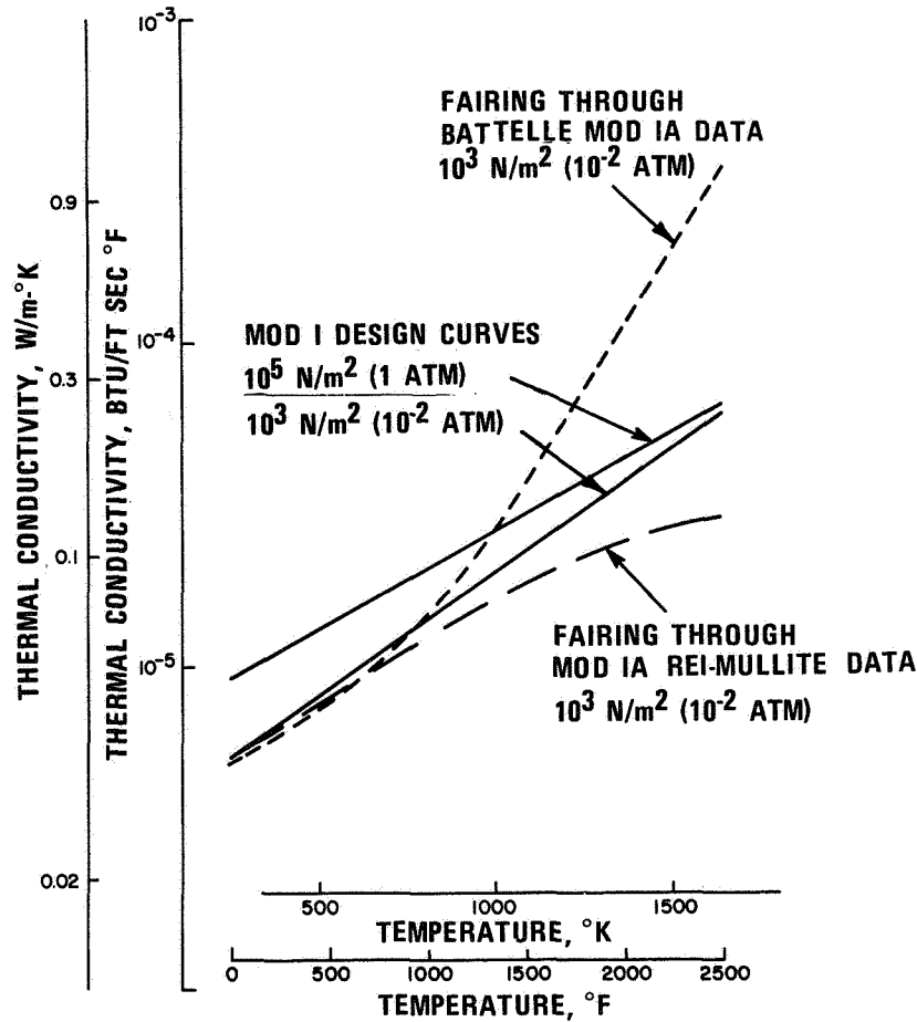
THERMAL CONDUCTIVITY DESIGN CURVES
