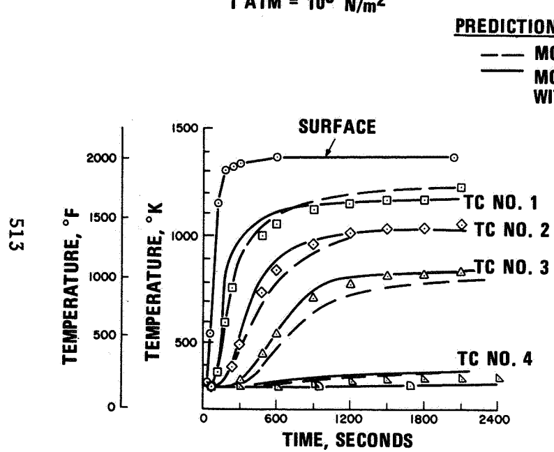
IN-DEPTH TRANSIENT RESPONSE OF MOD IA REI-MULLITE FROM GE-RESD TESTS
