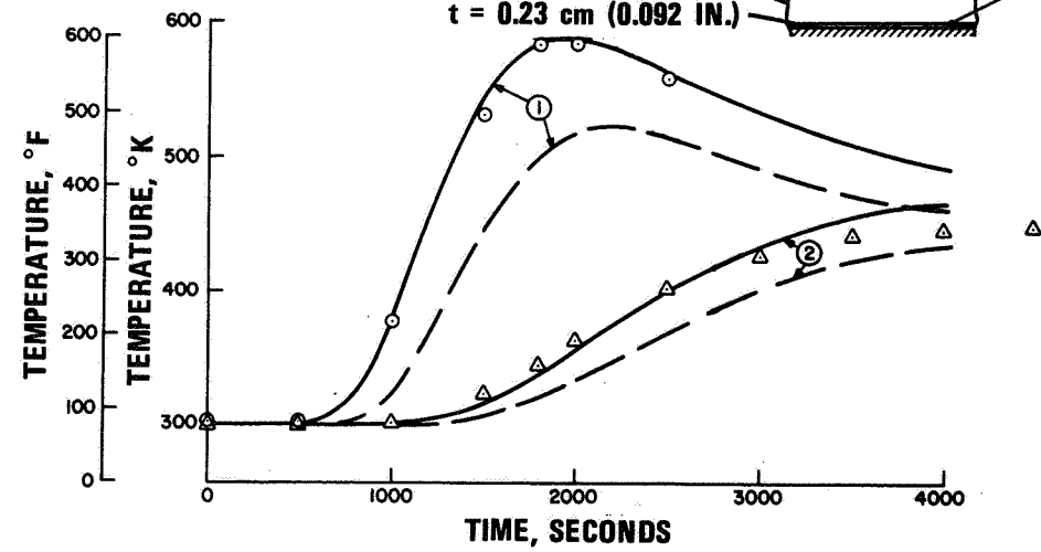
REI/BOND AND BOND/STRUCTURE TRANSIENT RESPONSE FOR NASA-MSC AREA 2P PROTOTYPE PANEL
