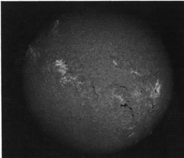
Figure 2 Solar Image in H-Alpha
