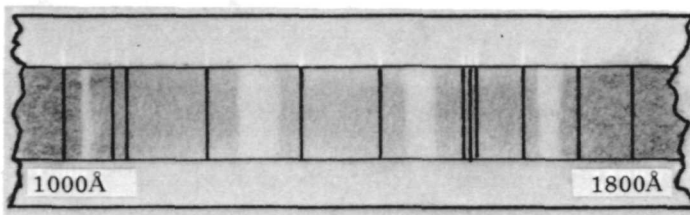
Figure 5 Spectrograph Data
