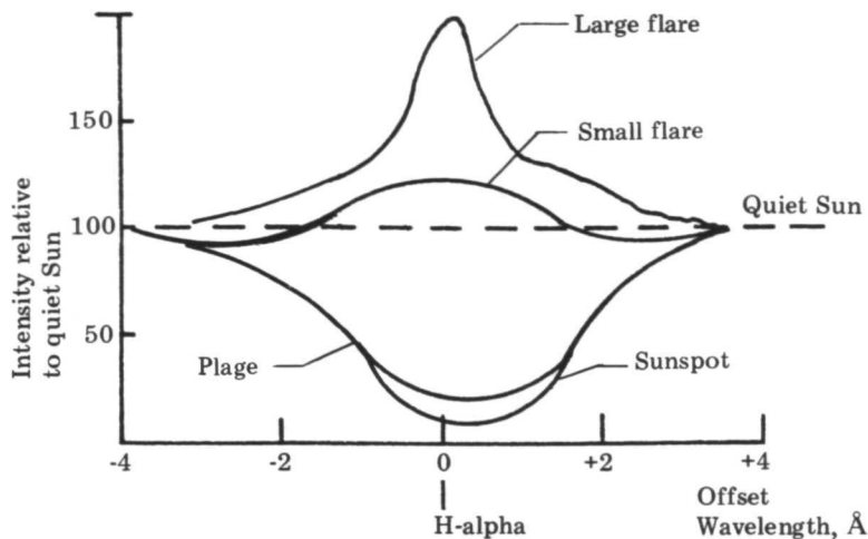
Figure 3 H-alpha Across Solar Phenomena
