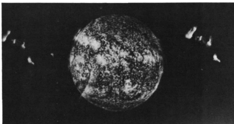
Figure 6 Spectroheliograph Data (from High Altitude Rocket Flight 9-22-68)
