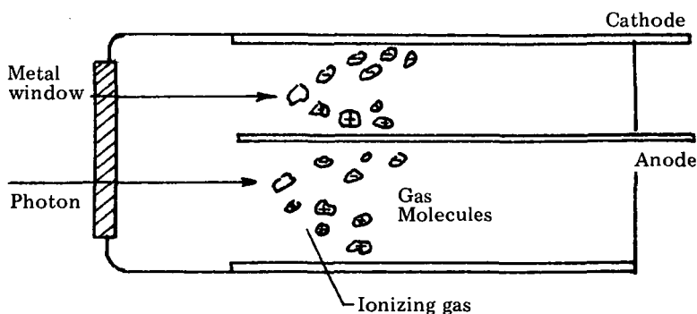
Proportional counter tube
