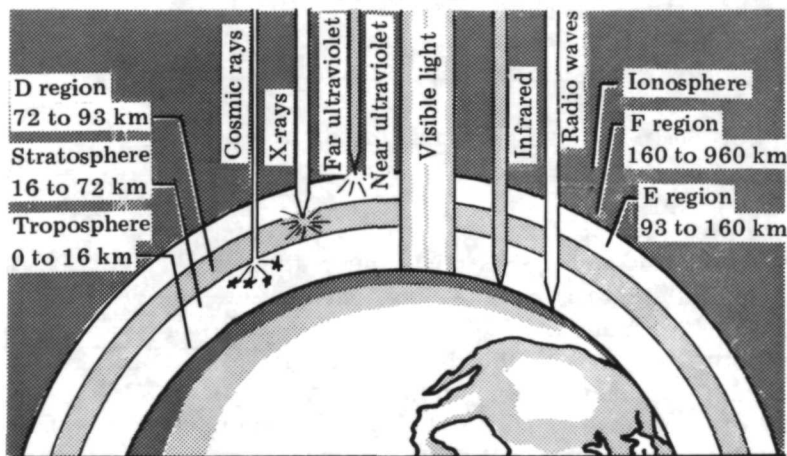
Figure 1 Atmospheric Absorption of Radiation
