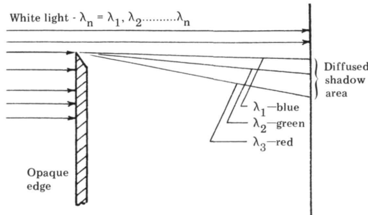
Diffraction of White Light Passing Over an Opaque Edge
