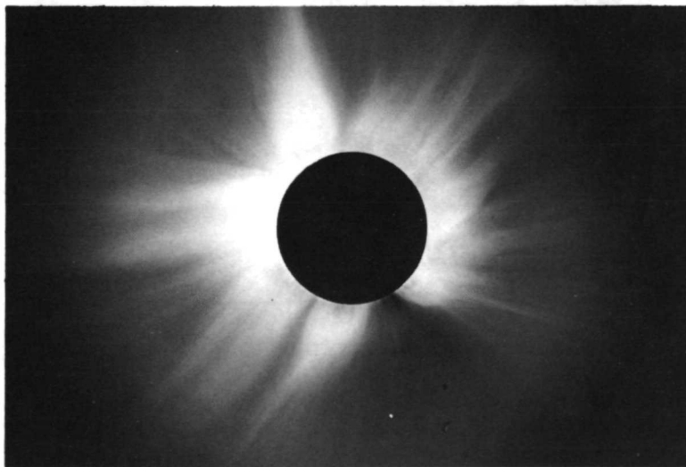
B 1970 Eclipse
