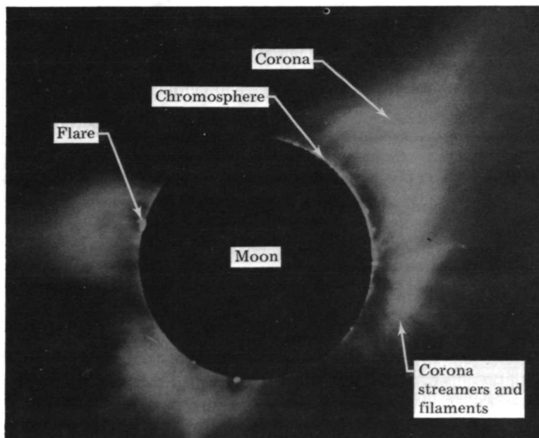
Near Corona Out 1 Solar Diameter Recorded during Eclipse
