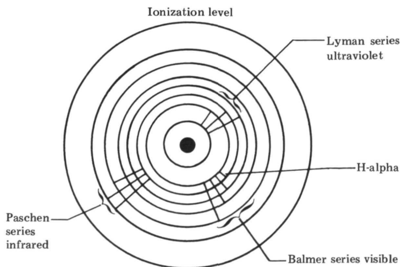
Figure 1 Hydrogen Series
