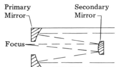
Cassegrain Telescope
