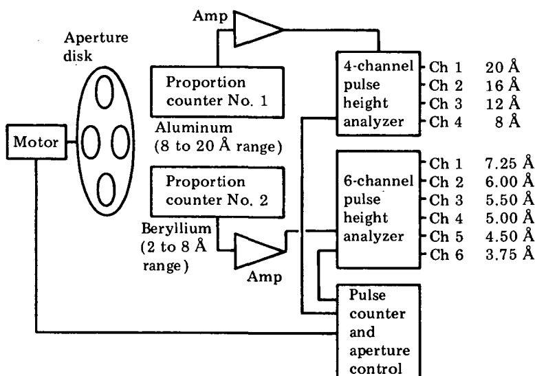
X-ray Event Analyzer
