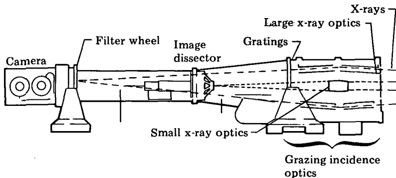
Plan of X-ray Telescope
