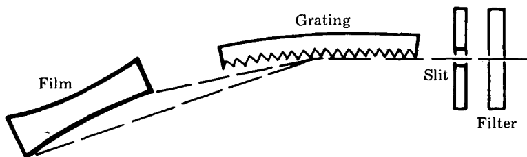
Optical Scheme of Extreme Ultraviolet Spectrograph
