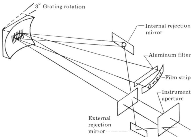
Figure 3 Optical System of the Spectroheliograph
