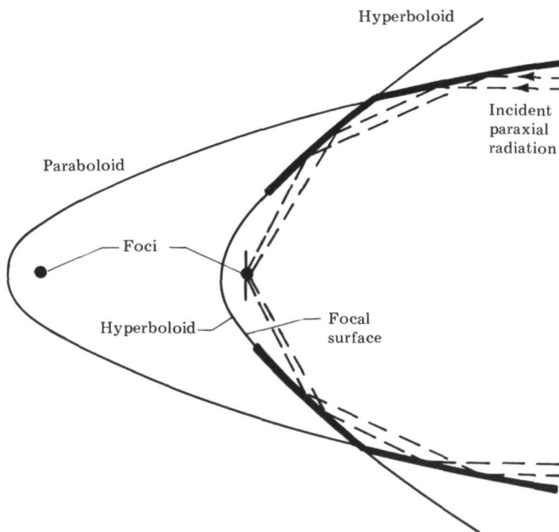
Grazing Incidence Telescope Geometry
