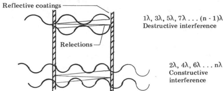
Figure 4 Interferometer Reflections
