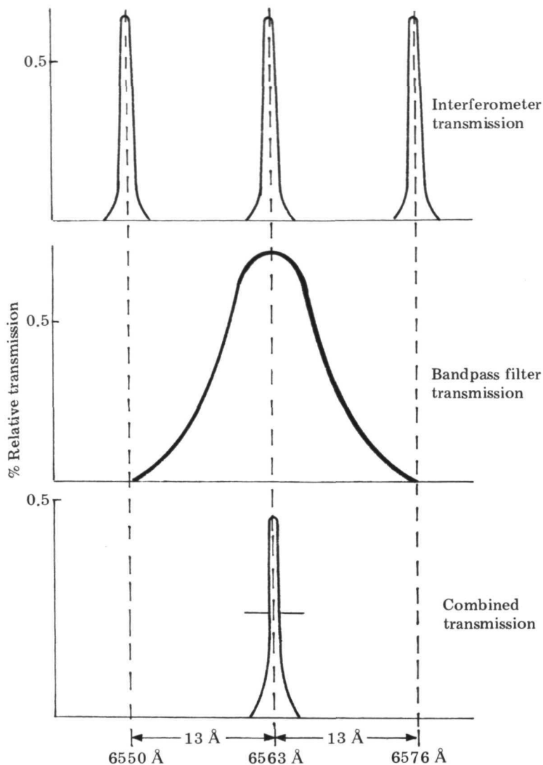
Figure 5 Interferometer Transmission
