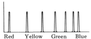
Interferometer Output in White Light
