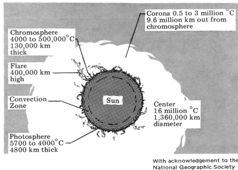
Figure 1 Solar Zones
