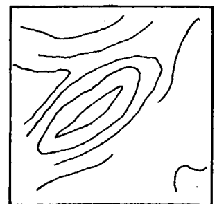
Reconstructed ultraviolet-scanning image
