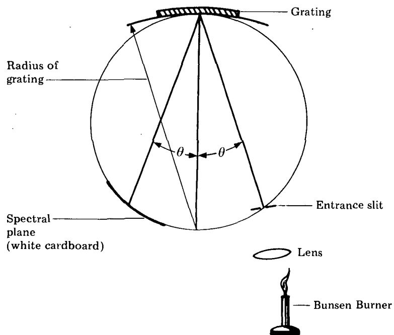
Figure 7 Experiment Layout
