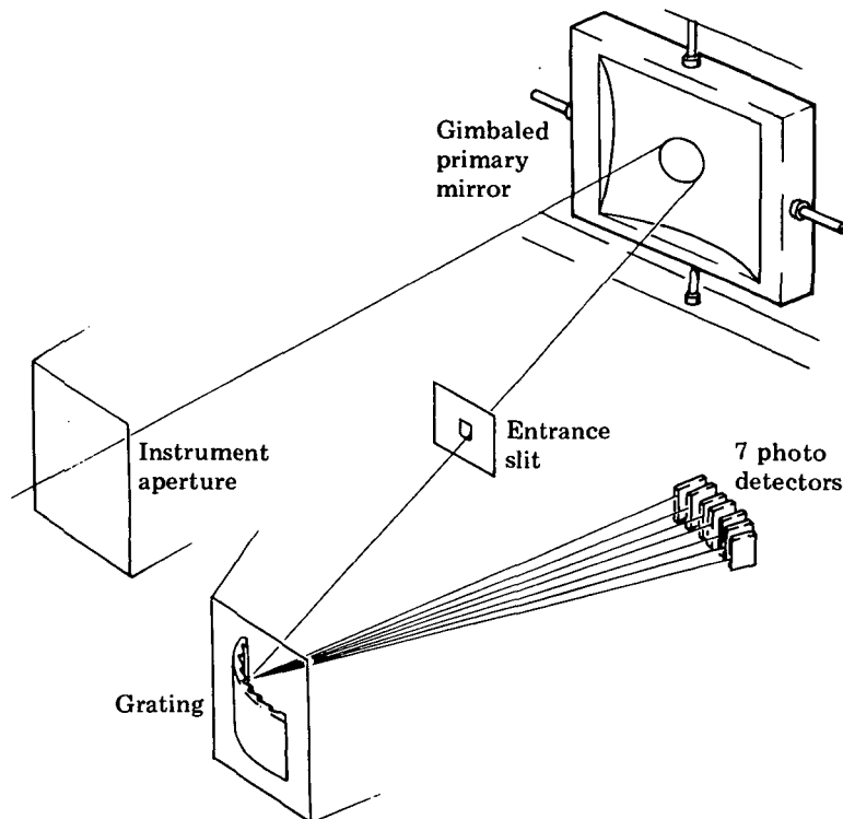
Optical Scheme of Ultraviolet Scanning Polychromator—Spectroheliometer
