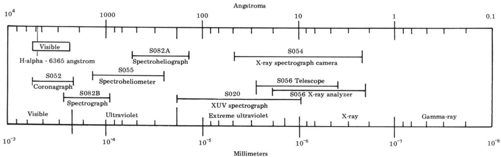
Figure 2 ATM Spectral Range
