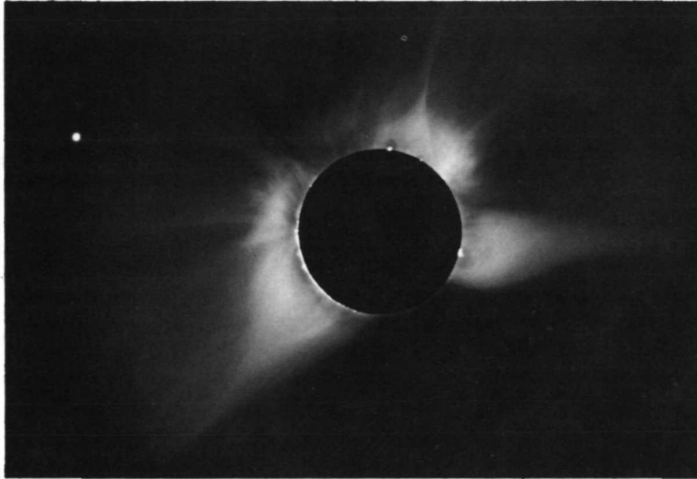
A 1966 Eclipse
