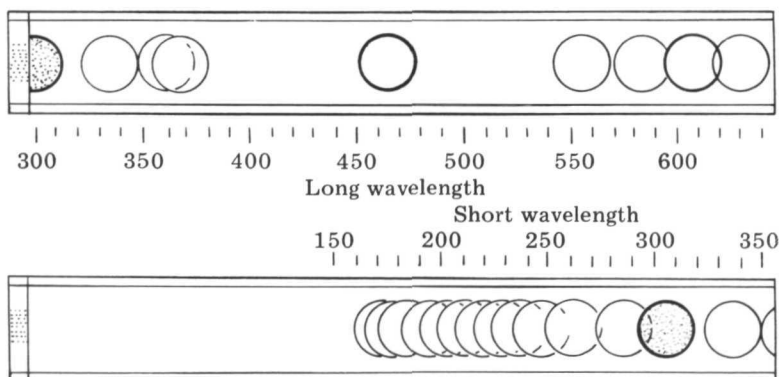
Figure 4 Diffracted Solar Images
