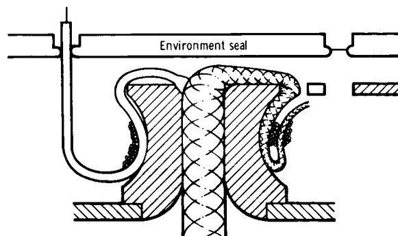
Figure 15. - Connector/cable joint.
