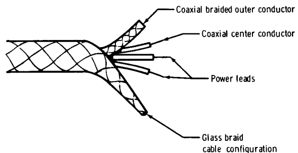
Figure 14.. - Cable configuration.
