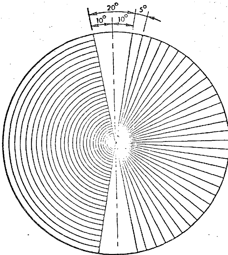
Figure 2. Detector geometry
