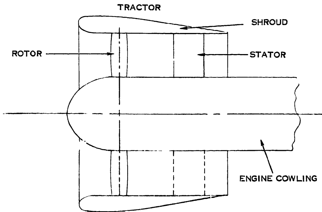
FIGURE 3. Q-FAN COMPONENTS
