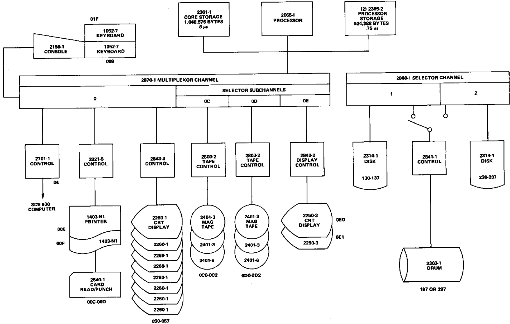
Figure 3.5-1. Equipment Configuration: IBM System 360, Model 65
