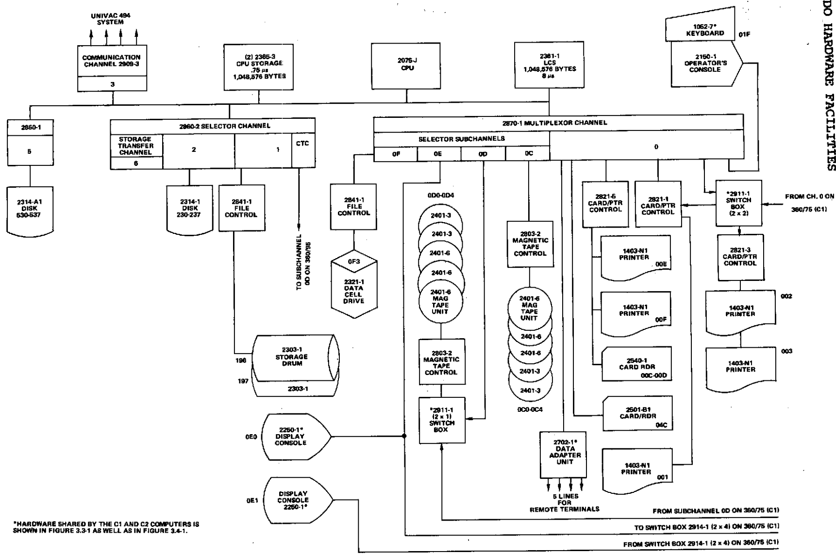
Figure 3.4-1. Equipment Configuration: IBM 360 System, Model 75 (C2)
