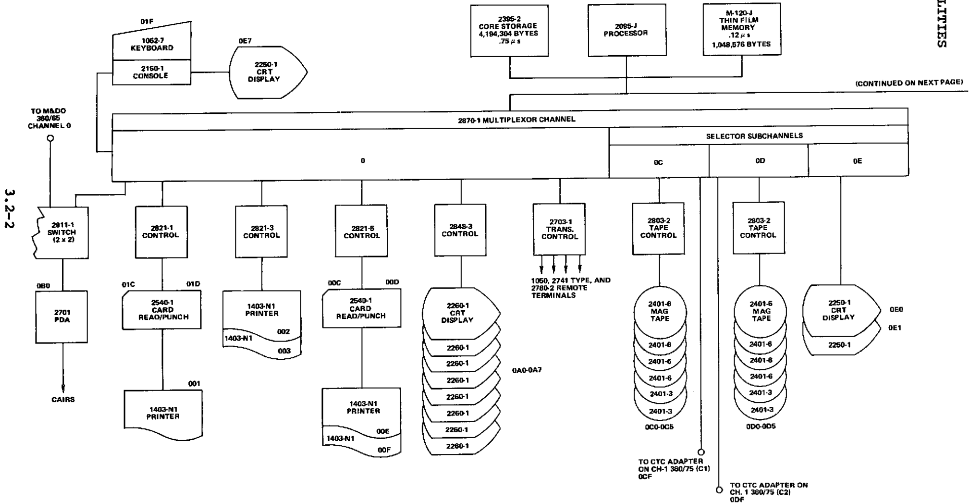
Figure 3.2-1. Equipment Configuration: IBM 360 System, Model 95 (Sheet 1 of 2)
