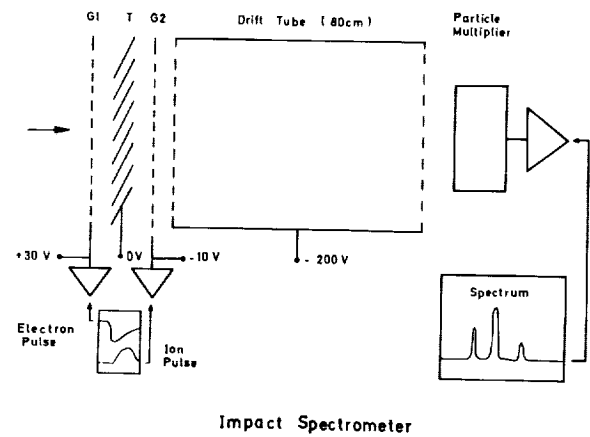
FIGURE 2.—Helios dust-detector schematic diagram.
