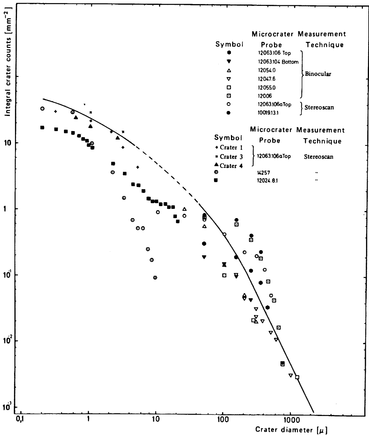
FIGURE 7.—Microcrater distribution on various lunar samples.
