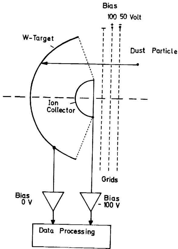
FIGURE 1.—HEOS dust-detector schematic diagram.
