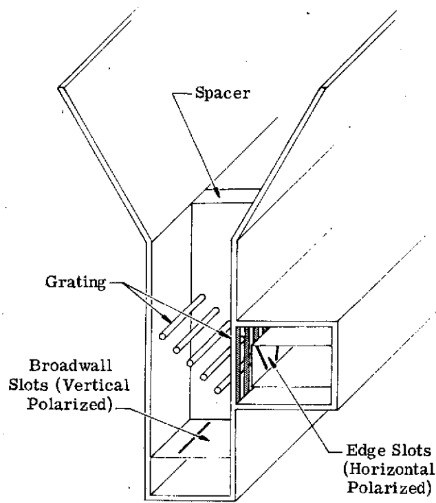
FIGURE 15. DUAL POLARIZED SLOT ARRAY (X-BAND)
