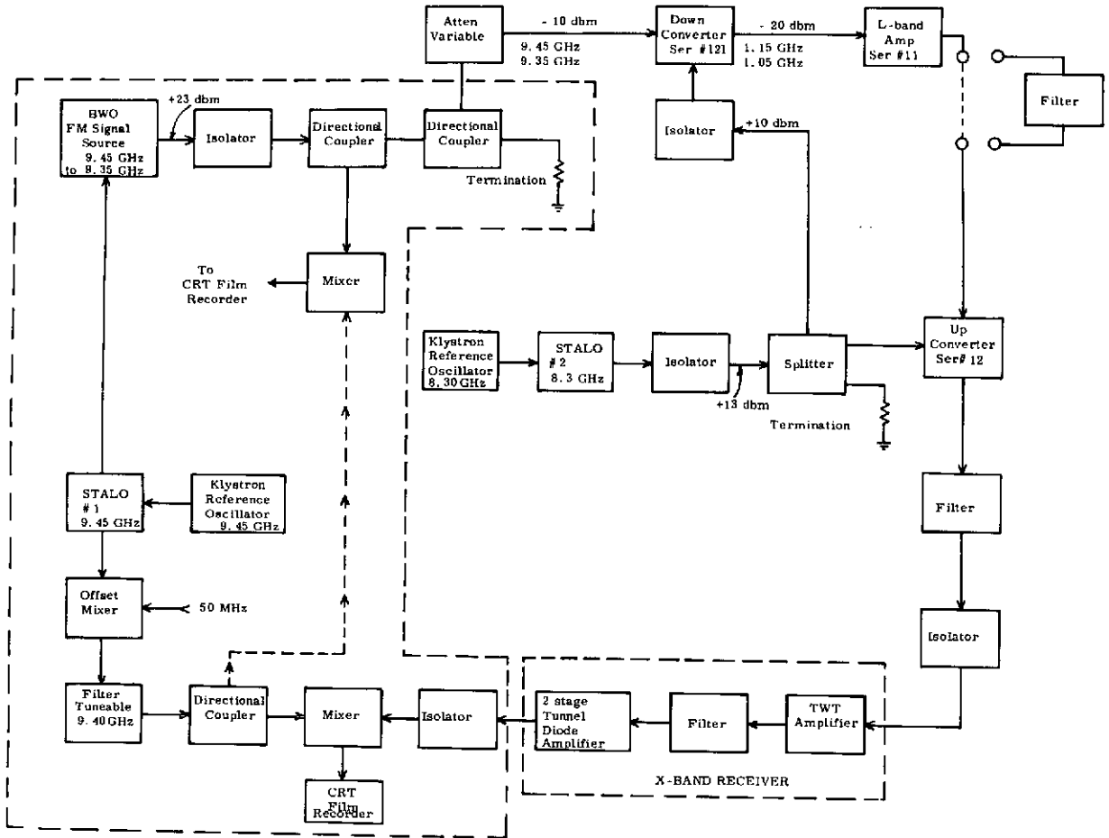
FIGURE 2. TEST - BLOCK DIAGRAM - X TO L TO X CONVERSION CONFIGURATION
