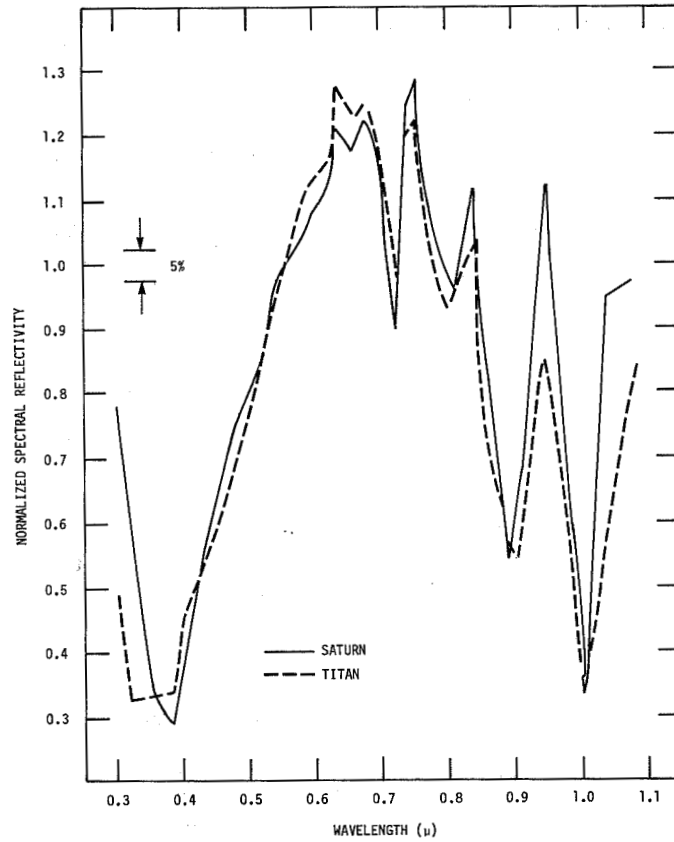
Figure 2-17. The spectral reflectance curve of Titan compared with that of Saturn's equatorial belt, scaled to unity at 0.56 \mu\text{m} . After McCord et al. (1971). Reprinted from The Astrophys. J. , 165: 422, with permission of The University of Chicago Press. © 1971. The University of Chicago. All rights reserved. Printed in U.S.A. (The turn-up of the Titan spectrum at 0.3 \mu\text{m} is probably spurious.)
