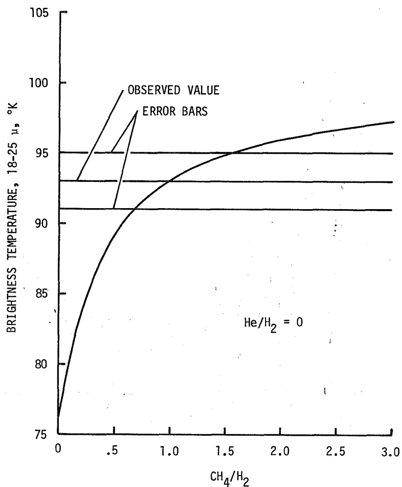
Figure 2-27. Theoretical brightness temperatures applicable to the 20 \mu\text{m} observation as a function of the methane-to-hydrogen ratio. The observed value with its mean and extreme values, permitted by the quoted error bars, is indicated by the horizontal lines. No helium is present in the model atmospheres. After Pollack (1973). Reprinted from Icarus , 19:50, with permission of Academic Press, Inc. Copyright © 1973 by Academic Press, Inc. All rights of reproduction in any form reserved.
