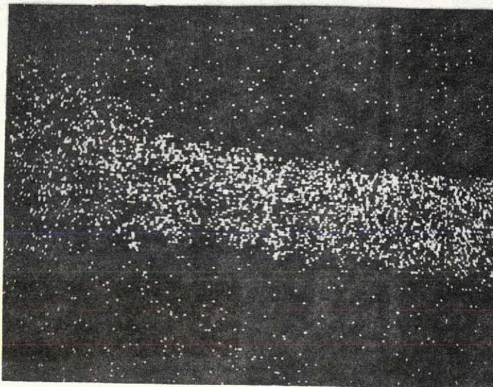
CHLORINE X-RAYS
