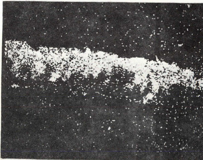
SILICON X-RAYS
