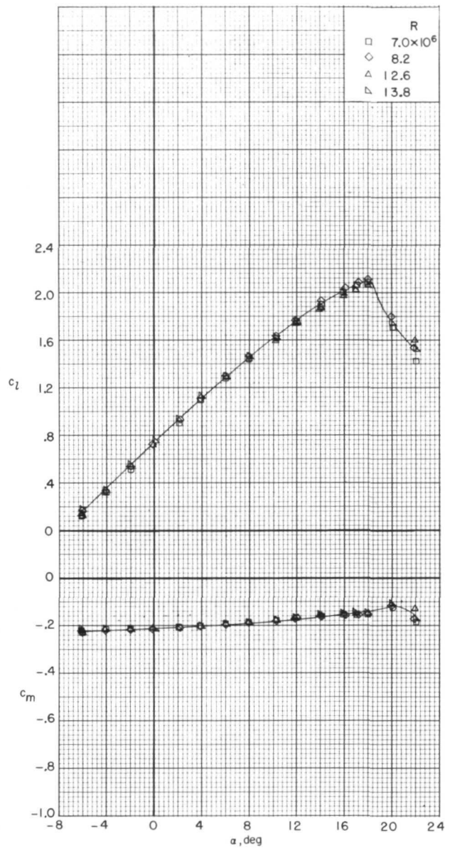
(f) Slot entry 3 sealed; \delta_f = 0^\circ ; M = 0.23 .
