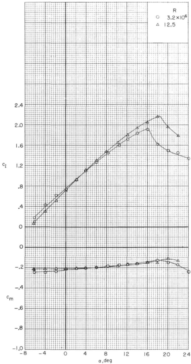
(e) Slot entry 3; \delta_f = 0^\circ ; M = 0.23 .
