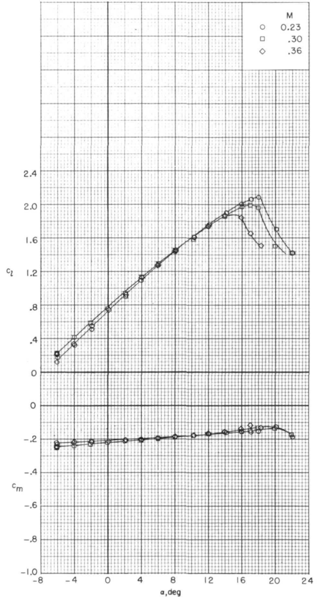
NACA 6716 airfoil
