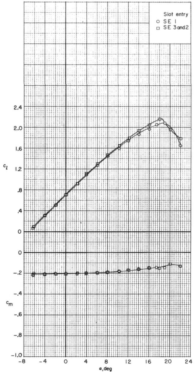
(j) \delta_f = 0^\circ ; R \approx 12 \times 10^6 ; M = 0.23 .
