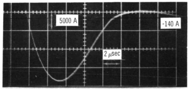
Figure 23. - Simulated thruster arc current pulses at atmospheric pressure.
