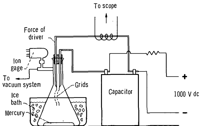
Figure 4. - Apparatus used to simulate ion thruster arc.
