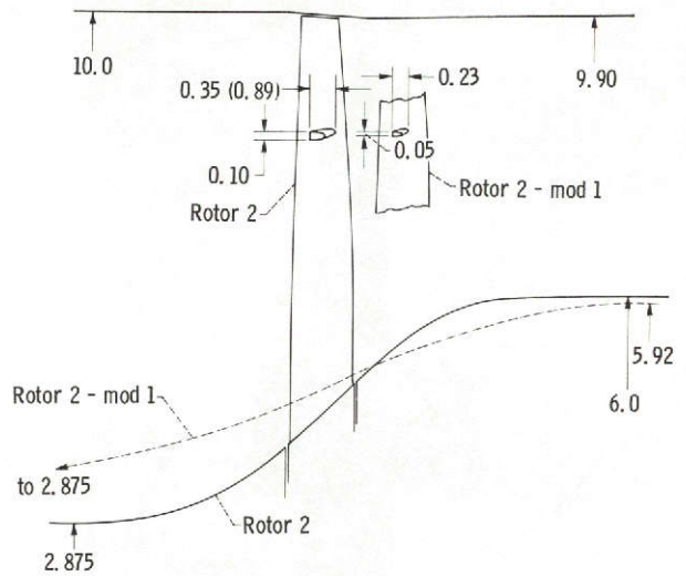
(b) Side-view schematic. (All dimensions are in inches.)
