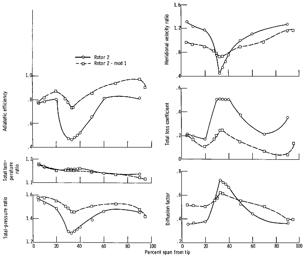
Figure 11. - Radial distribution of performance parameters for rotor 2 and rotor 2 - mod 1 at design speed and near-stall weight flow.
