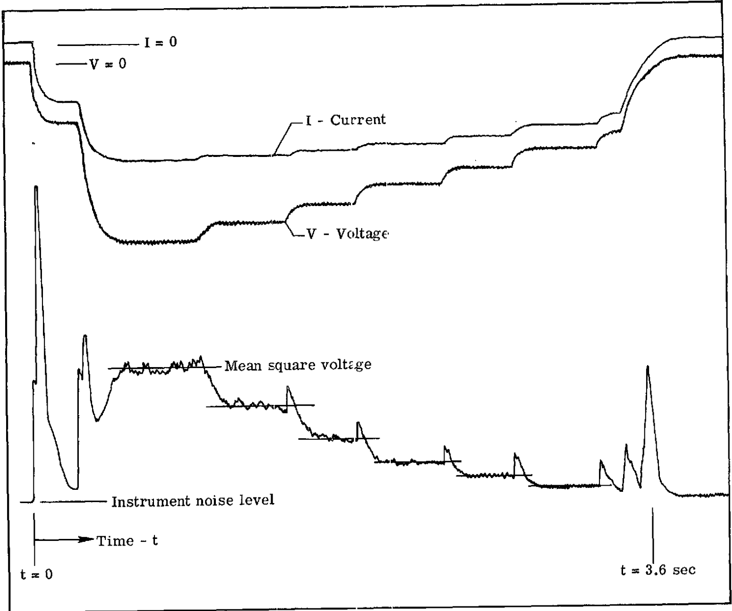
Figure 2.- Oscilloscope record of hot-wire signals.
