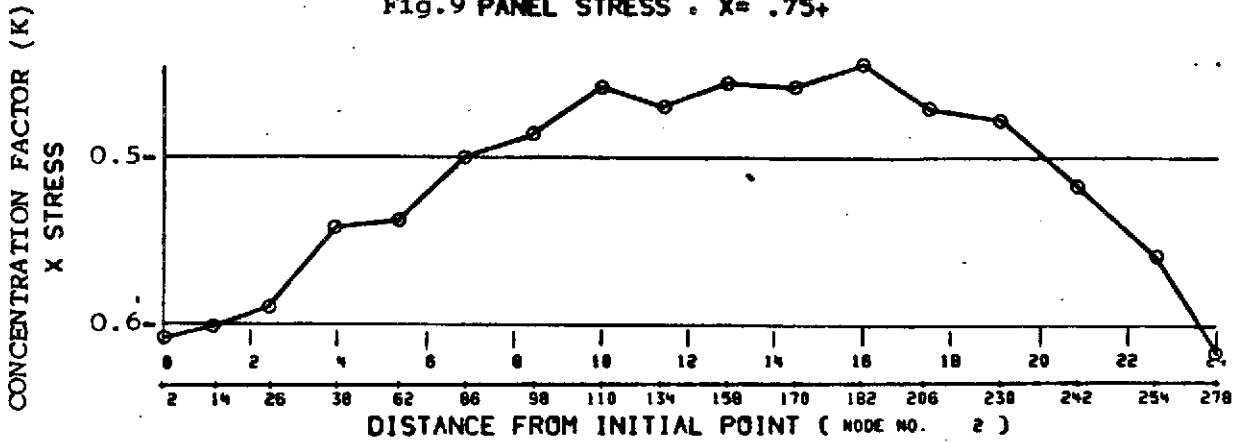
Fig. 9 PANEL STRESS . X= .75+
