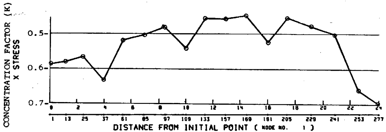
Fig. 10 PANEL STRESS . X= 0.0+
