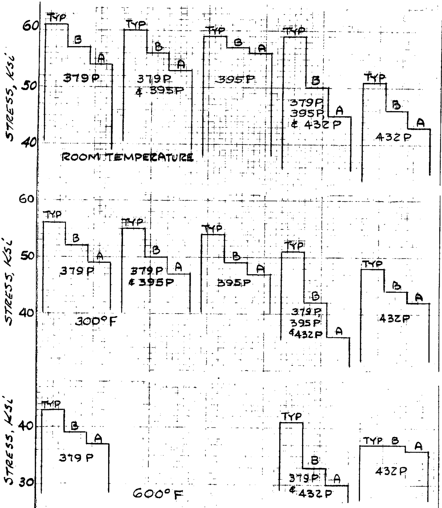
FIGURE 18 COMPRESSIVE YIELD STRENGTH TRANSVERSE
