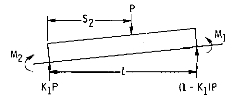
(c) Free body of pad.
