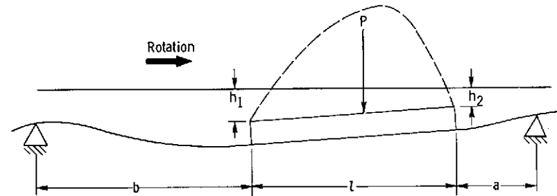
(a) Pad and flexible beam arrangement.
