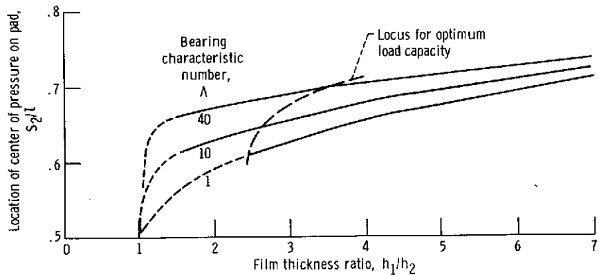
Figure 5. - Location of center of pressure as function of film thickness ratio and bearing characteristic number for flat, square slider (ref. 12).
