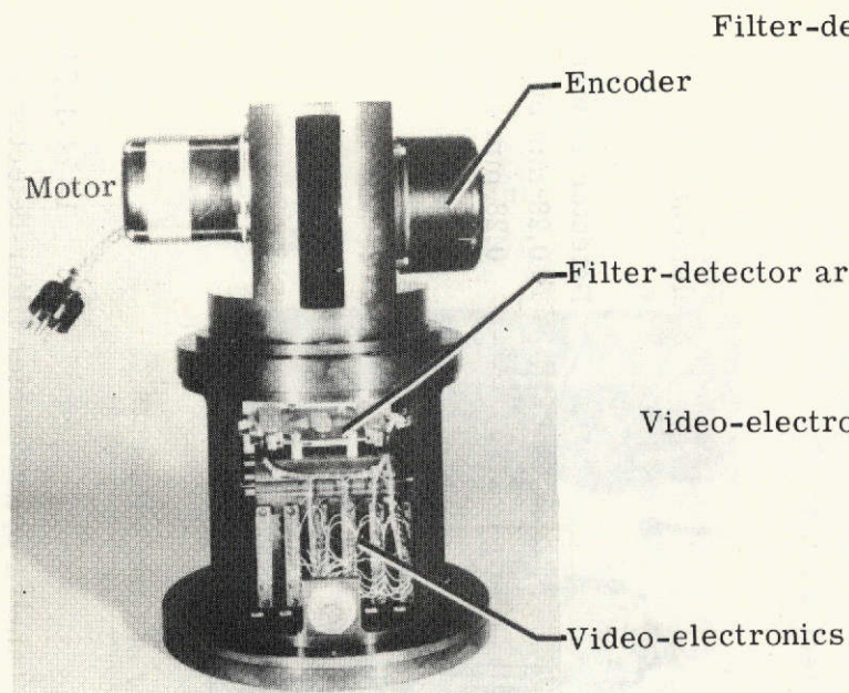
(a) Laboratory facsimile camera (without azimuth rotation base).
