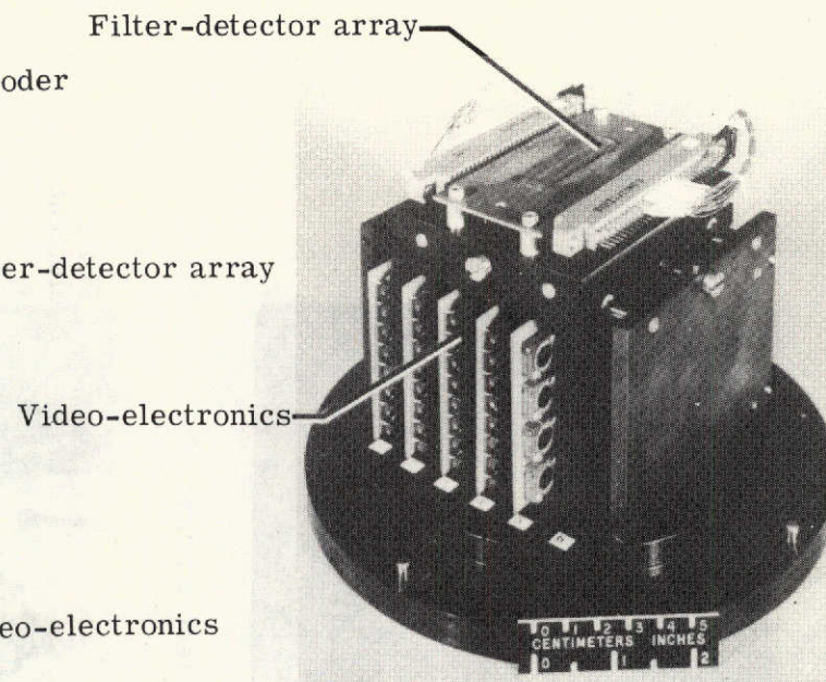
(b) Filter-photosensor array with signal multiplexing and amplifi- cation electronics.
