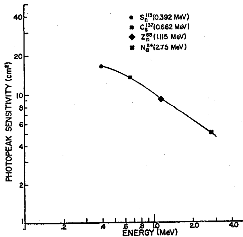
Figure II-2. Energy dependence of the detector sensitivity ( \text{cm}^2 ) for an axial parallel beam for four line sources.
