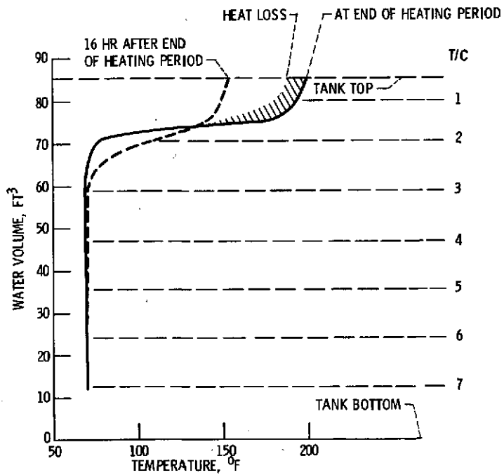
Figure 15. - Temperature distribution within tank after heating.
