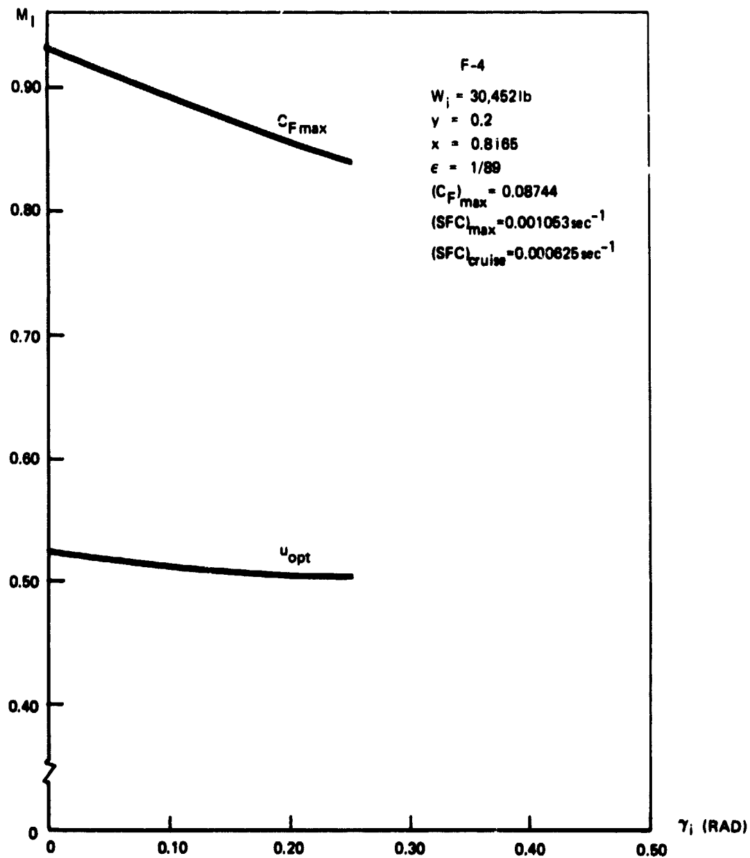
Figure 6.12. Fuel Cost for u_{\text{opt}} and C_{F\max} Initial Transitions for Various Initial Conditions at \gamma = 0.2
