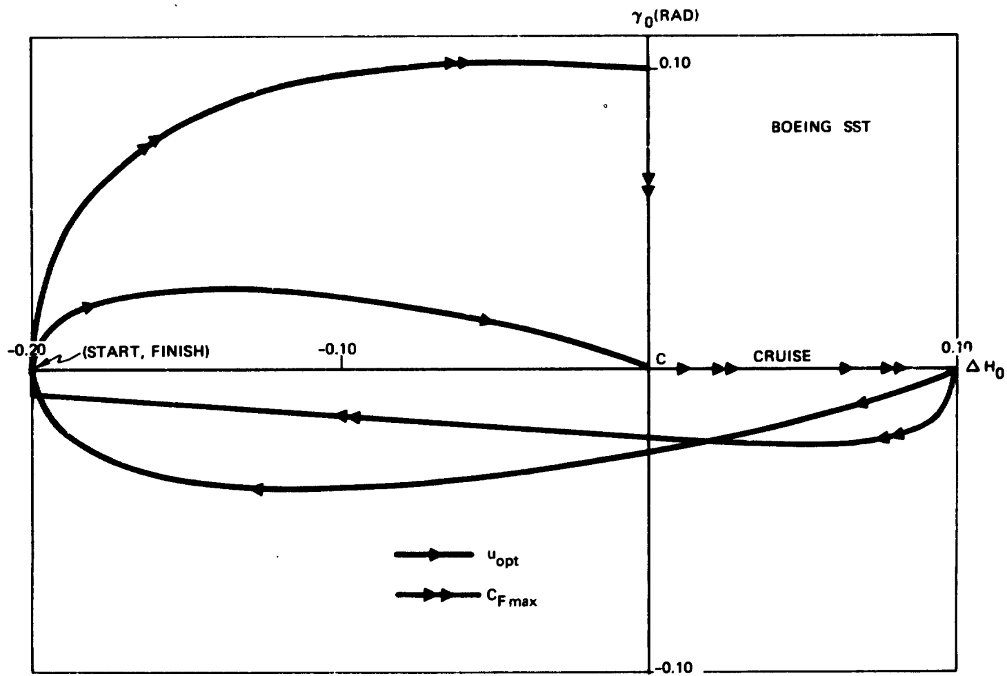
Figure 6.7. Climb, Cruise, Descent Trajectories for u_{opt} and C_{Fmax} Transitions
