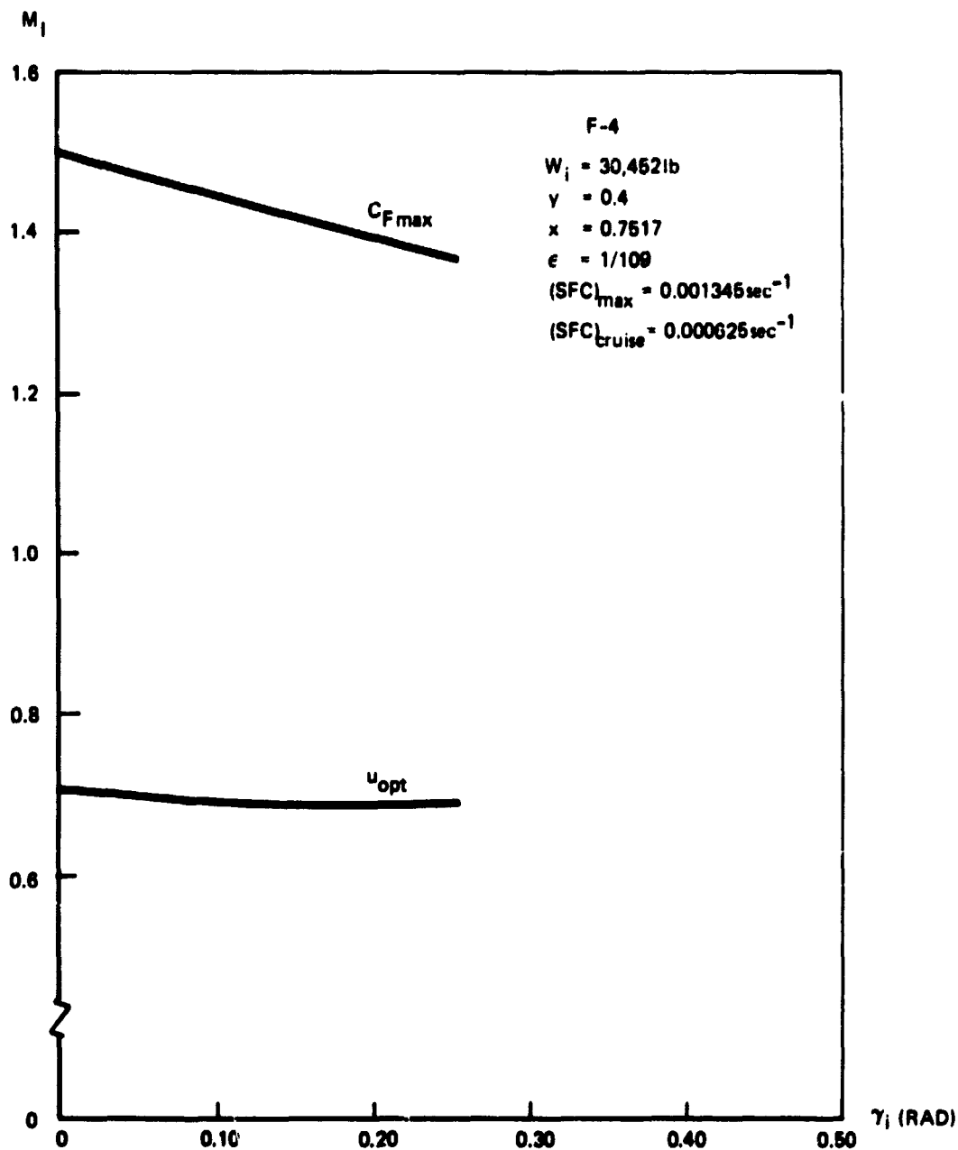
Figure 6.13. Fuel Cost for u_{\text{opt}} and C_{F\text{max}} Initial Transitions for Various Initial Conditions at \gamma = 0.4
