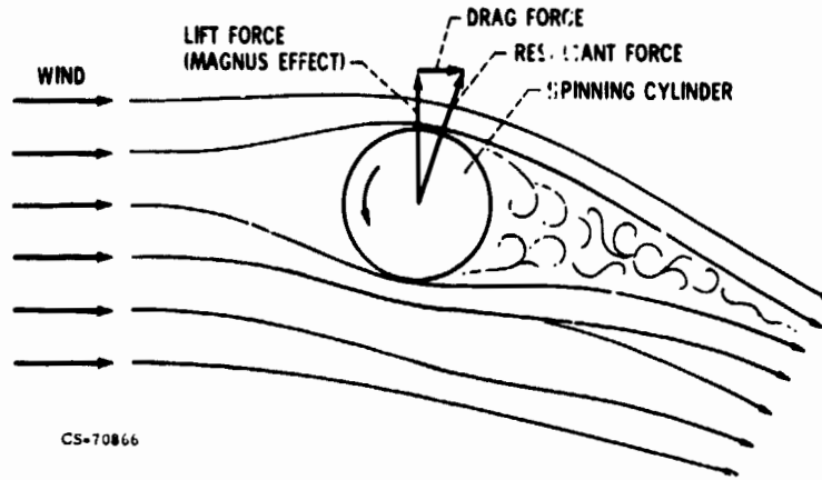
Figure 1(a). - The Magnus effect.
