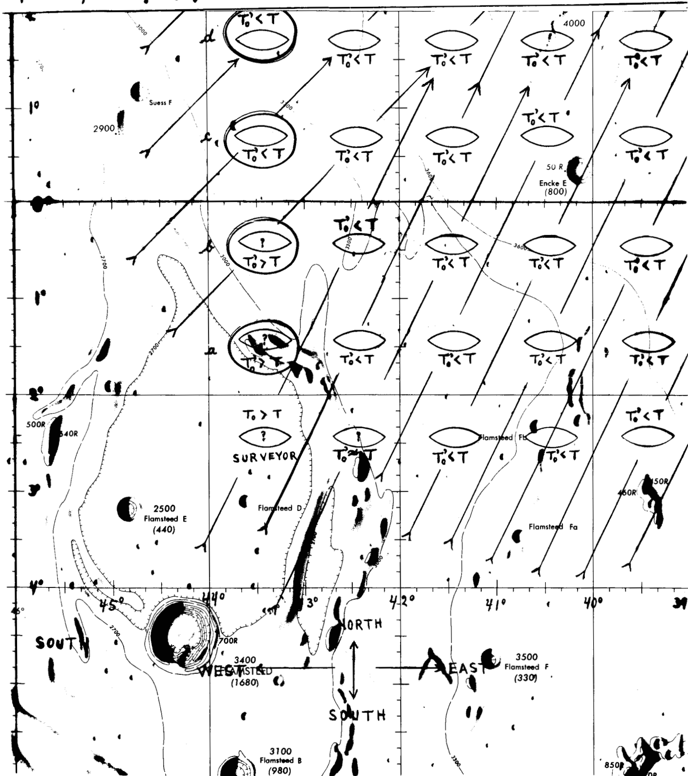
Predicted Temperatures as a Function of the Radial Lines of Major Craters - No. 1
