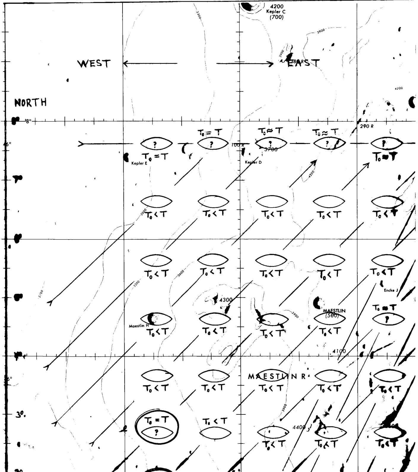
Predicted Temperatures as a Function of the Radial Lines of Major Craters - No.2
