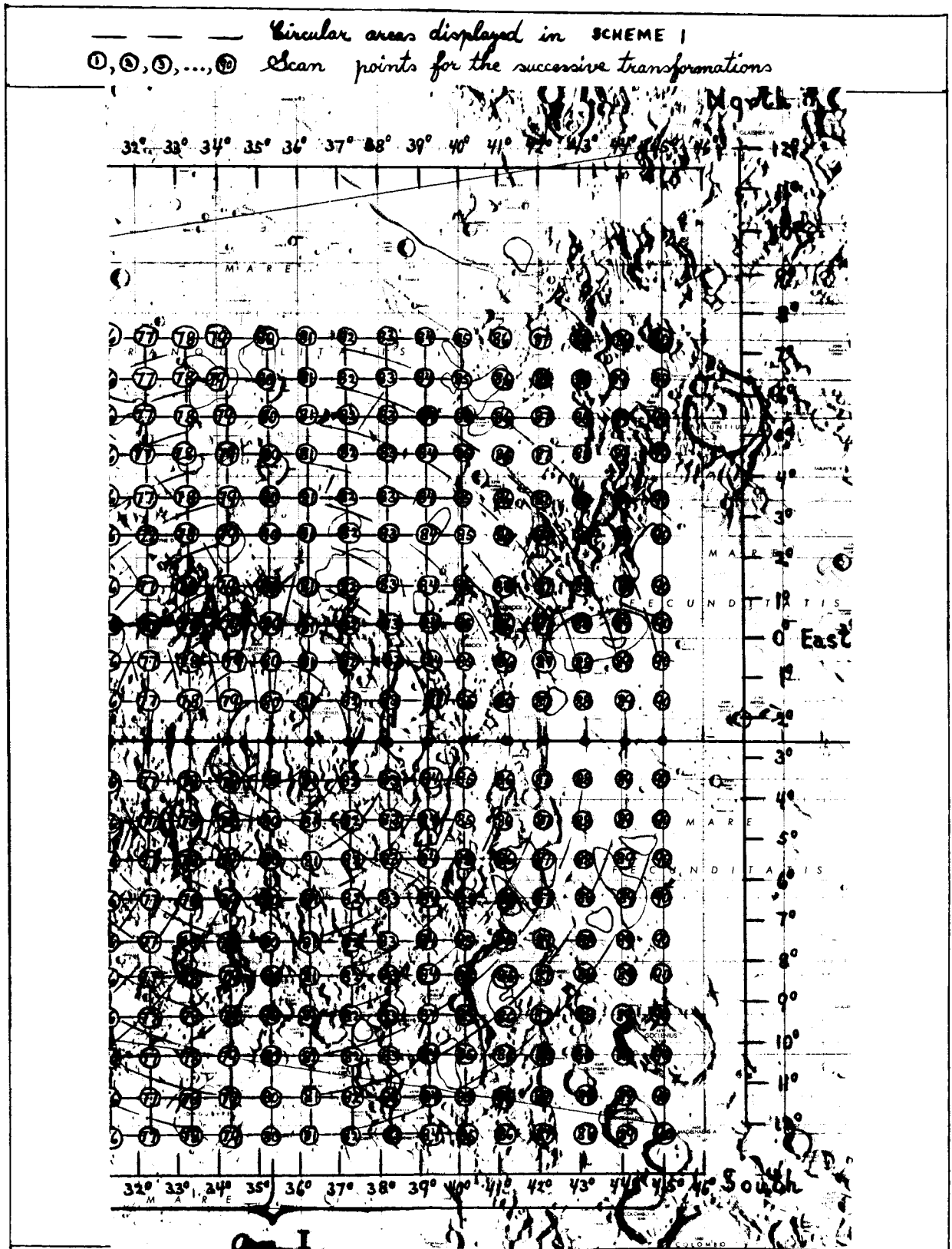
Map of the Moon Containing the Points To Be Observed, Whose Data Will Be Reduced by the Successive Transformation Method - Part V
