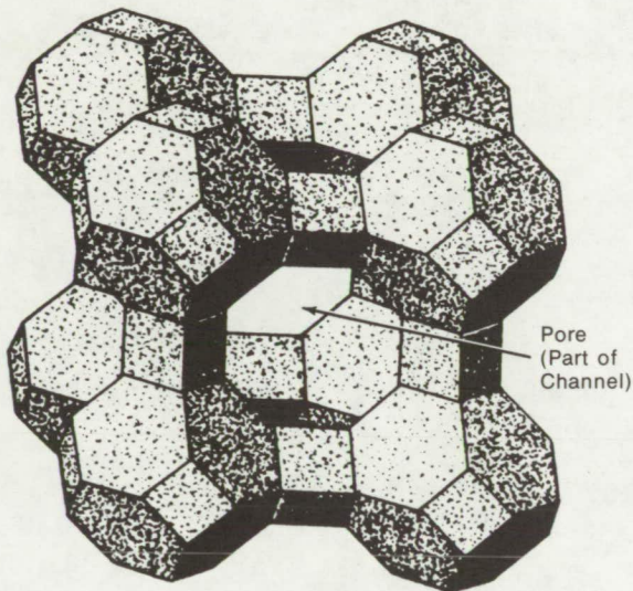
Figure 1. Sodalite Cage
