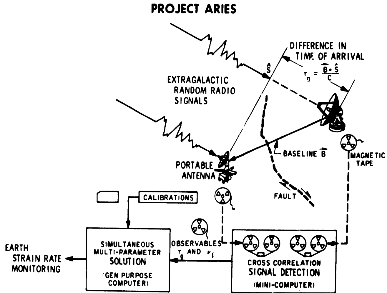
Figure 4. Sketch and Flow Diagram of a Working VLBI System for Earth Physics Using a Portable Antenna
