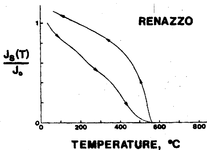
Fig. 42. J_s -T curve for an exceptional sample of Renazzo.
