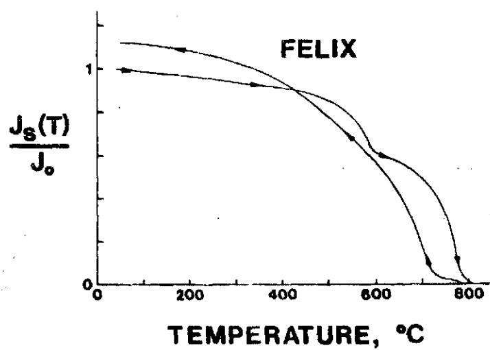
Fig. 52. J_s -T curve for Felix.
