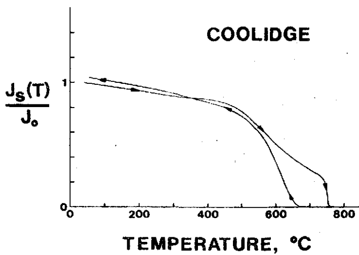
Fig. 56. J_S -T curve for Coolidge.
