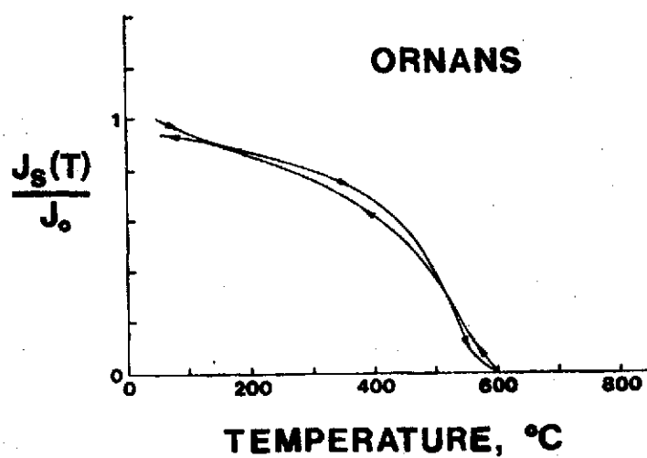
Fig. 50. J_s -T curve for Ornans.
