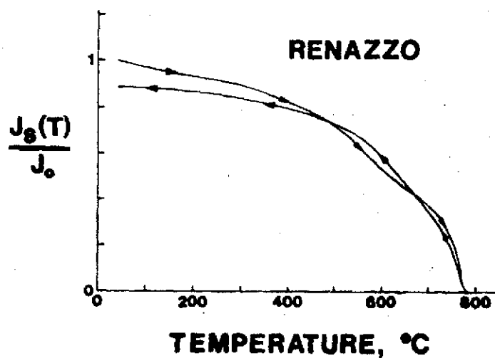
Fig. 41. J_s -T curve similar to several samples of Renazzo.
