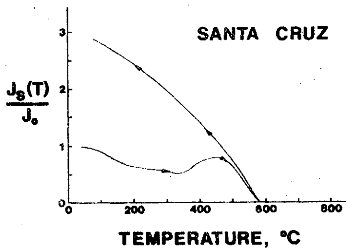
Fig. 31. J_S -T curve for Santa Cruz.
