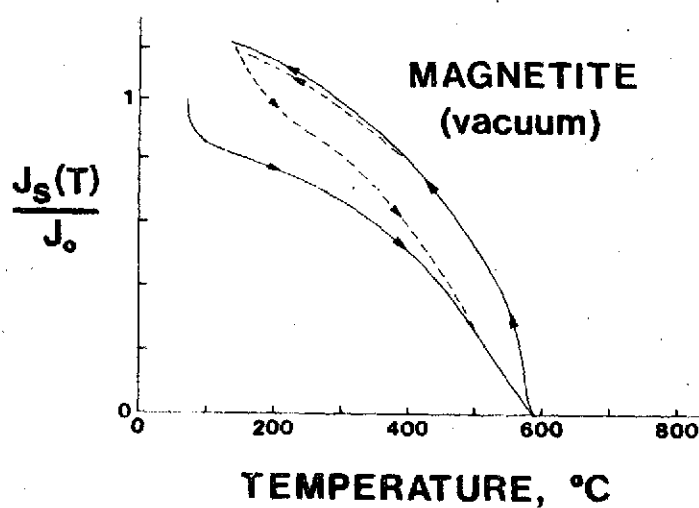
Fig. 10. J_s -T curve for synthetic magnetite run under vacuum ( 4 \times 10^{-4} torr). The broken curve indicates the second thermal cycle.
