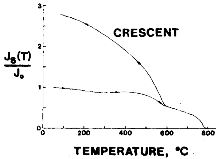
Fig. 25. J_S -T curve for Crescent.
