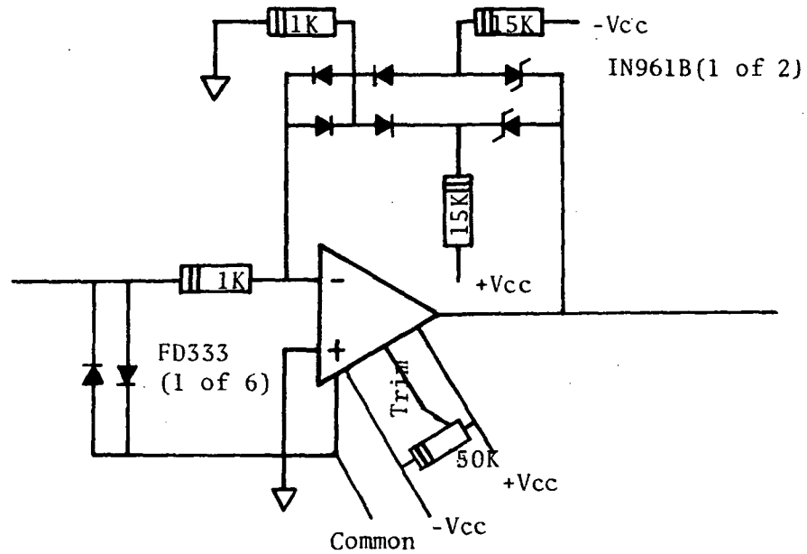
Figure 20 Over-Voltage and Latch-up Protection Circuits for Analog Devices 233L Op Amp
