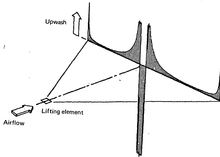
(a) UPWASH PRODUCED BY LIFTING ELEMENT
