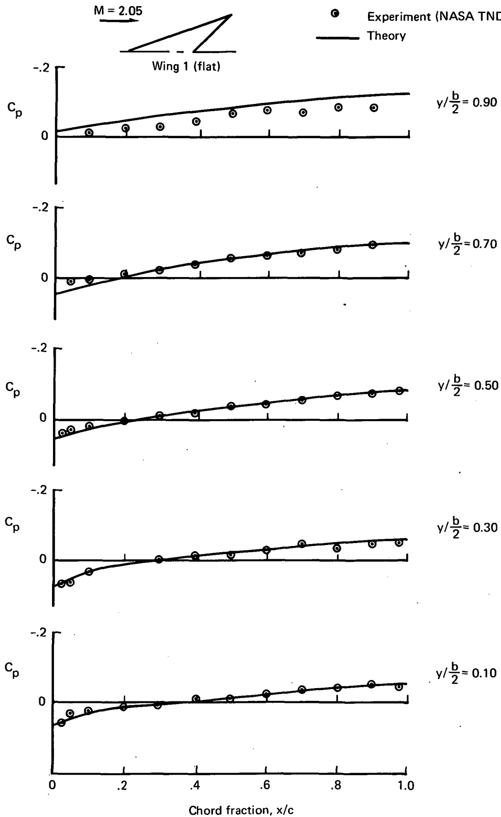
FIGURE 4.4-12.— THICKNESS PRESSURE COMPARISON ( C_p DUE TO THICKNESS ONLY)
