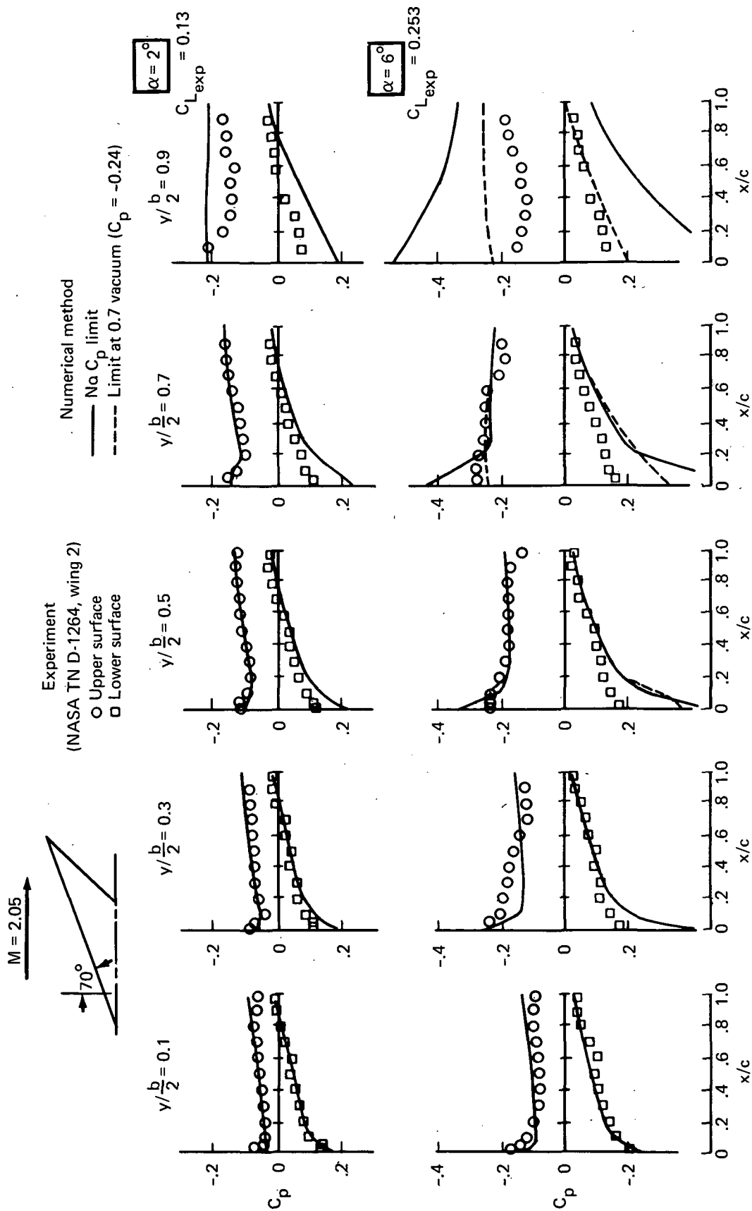
FIGURE 4.4-14.—PRESSURE COEFFICIENT COMPARISON, WING 2 (TWISTED AND CAMBERED WING, DESIGN C_L = .08 )
