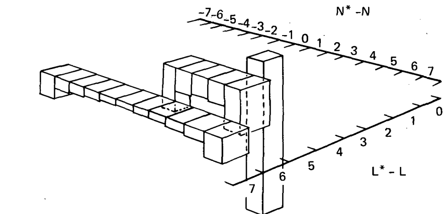
b) REPRESENTATIVE INFLUENCE FACTOR CHARACTERISTICS FIGURE 4.3-2.—THICKNESS PRESSURE INFLUENCE FUNCTION
