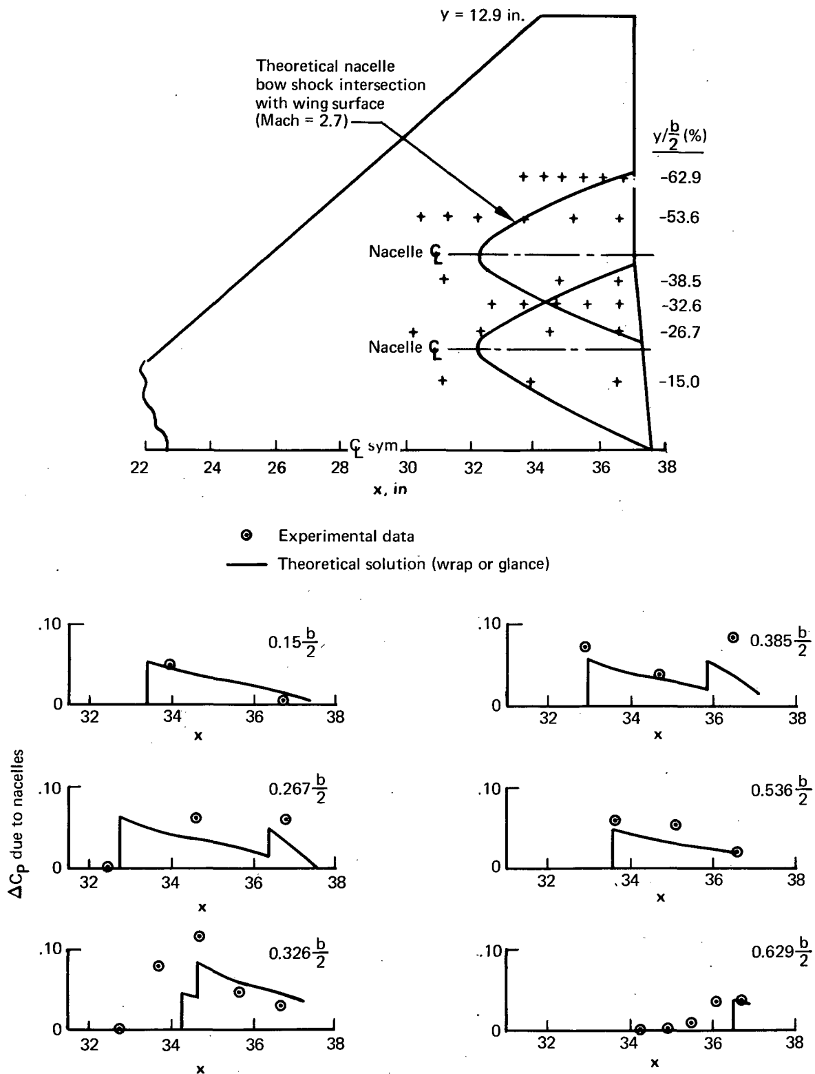
FIGURE 4.3-8.—NACELLE PRESSURE FIELD DATA, M = 2.7
