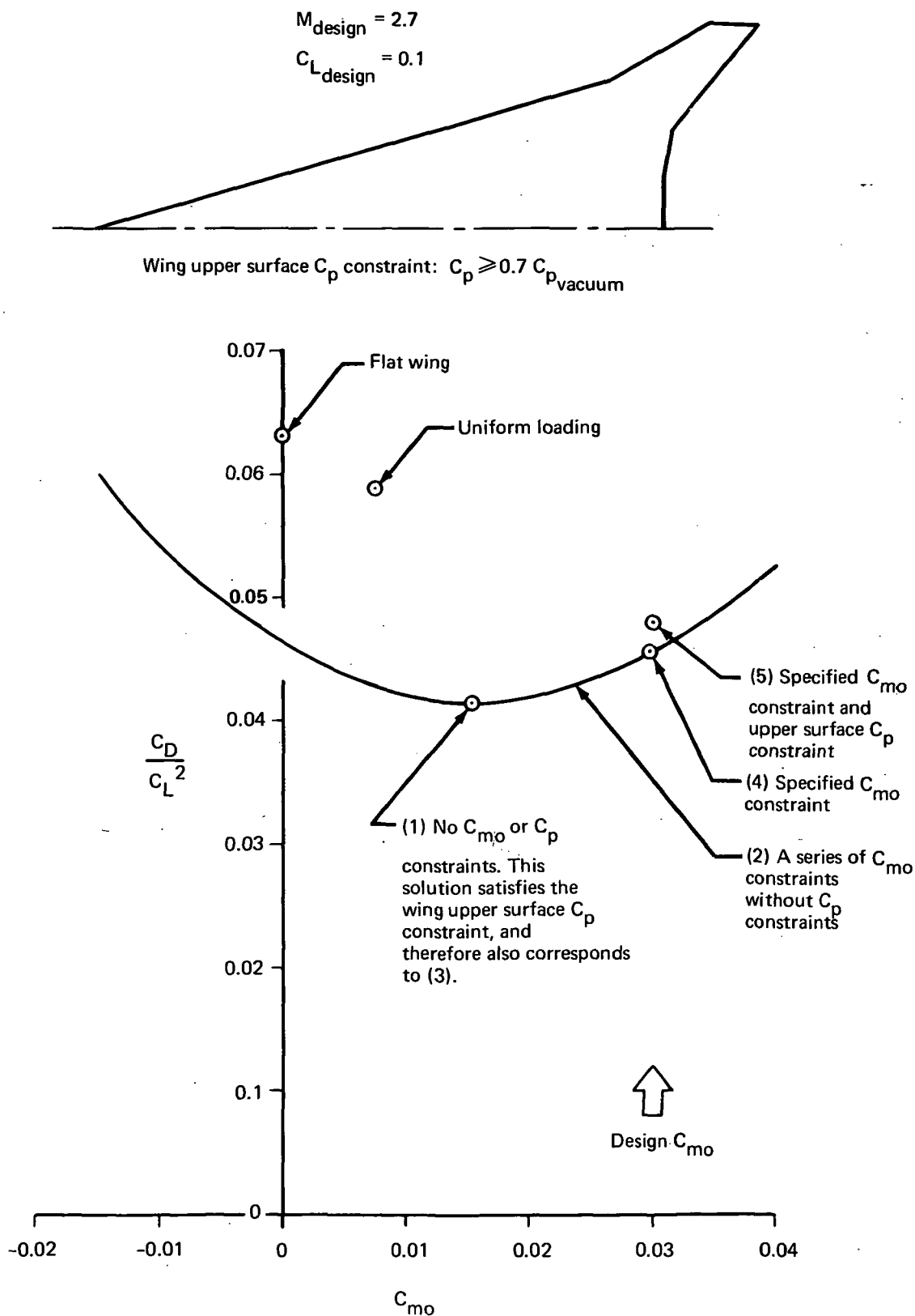
FIGURE 4.4-5.—TYPES OF LOADING SOLUTIONS
