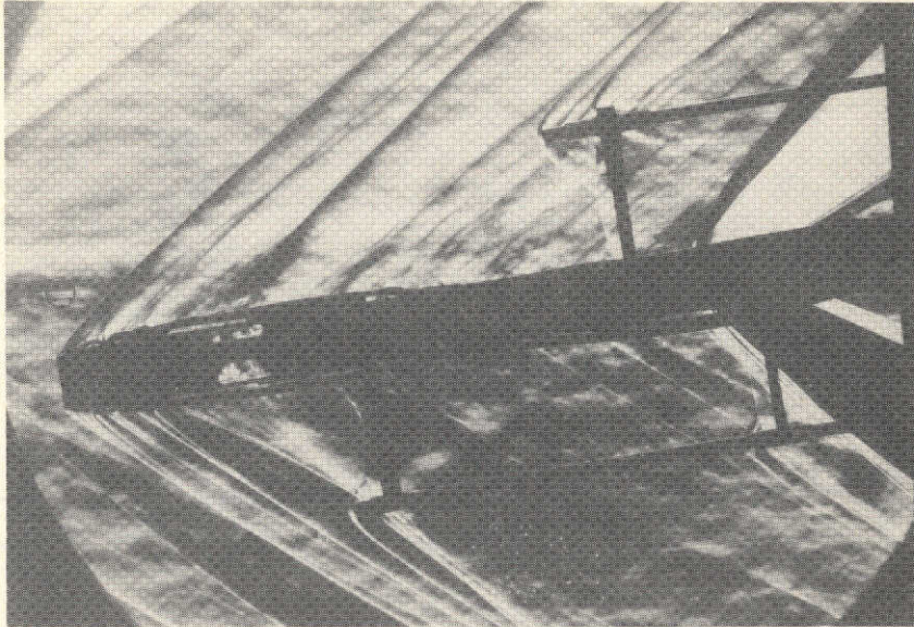
(a) Shock swallowed.
