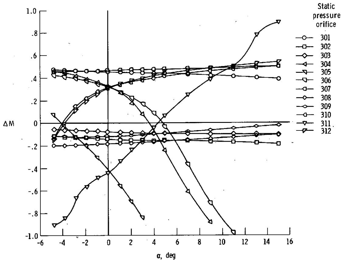
Figure 17. Mach number error versus angle of attack for the 300-series orifices in tip 3. Sleeve wide open; total pressure tube position = 7.5 cm (2.9 in.); Re \approx 16.4 \times 10^6 per m ( 5 \times 10^6 per ft); \beta \approx 0^\circ ; orifices 301 and 307 oriented in the horizontal plane.
