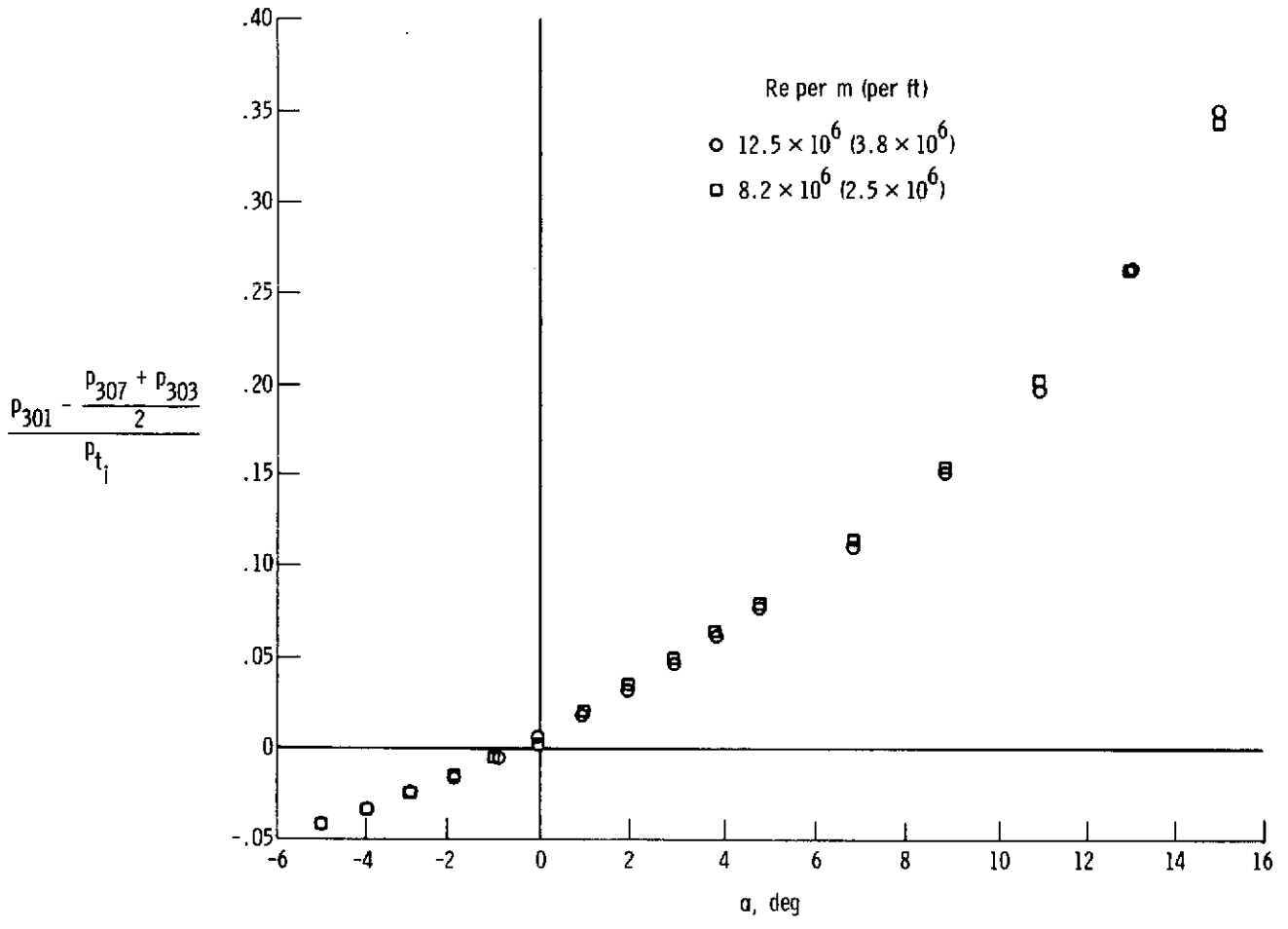
Figure 13. Calibration showing use of shock-swallowing probe to measure angle of attack. \beta \approx 0^\circ , tip 1.
