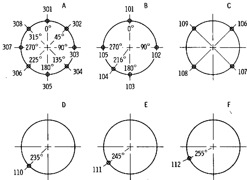
View looking downstream Static pressure orifice locations
