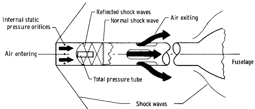
Shock-swallowing probe
