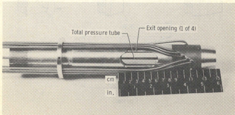
(b) Maximum exit opening.
