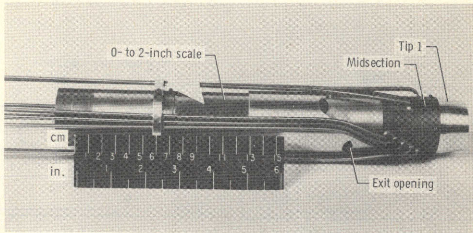
(a) Minimum exit opening.
