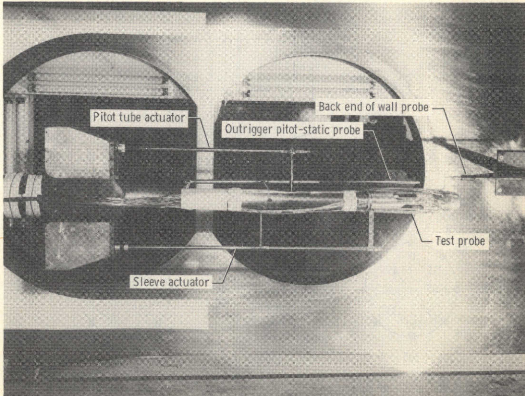
Figure 4. Probe mounted in wind tunnel.
