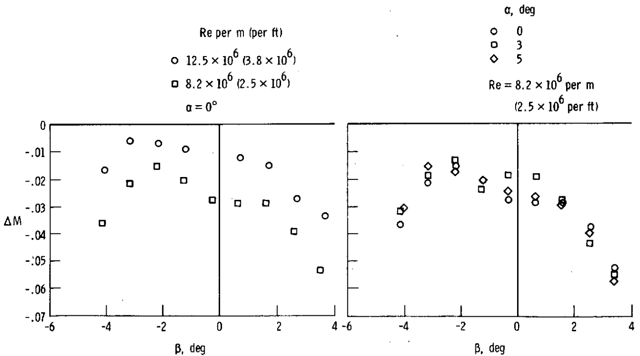
(b) Effect of angle of sideslip.
