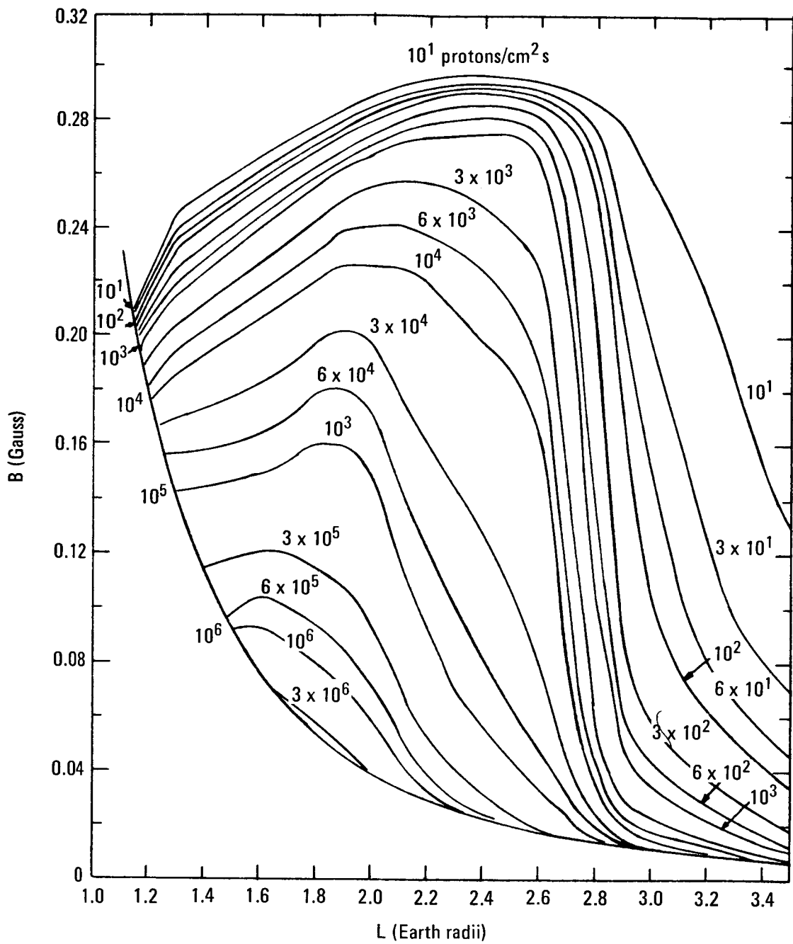
Figure 51.—Model AP6 omnidirectional proton flux ( E > 4 MeV) as function of B and L (ref. 117).
