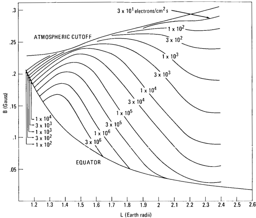
c. E > 1 \text{ MeV} , Epoch October 1967
