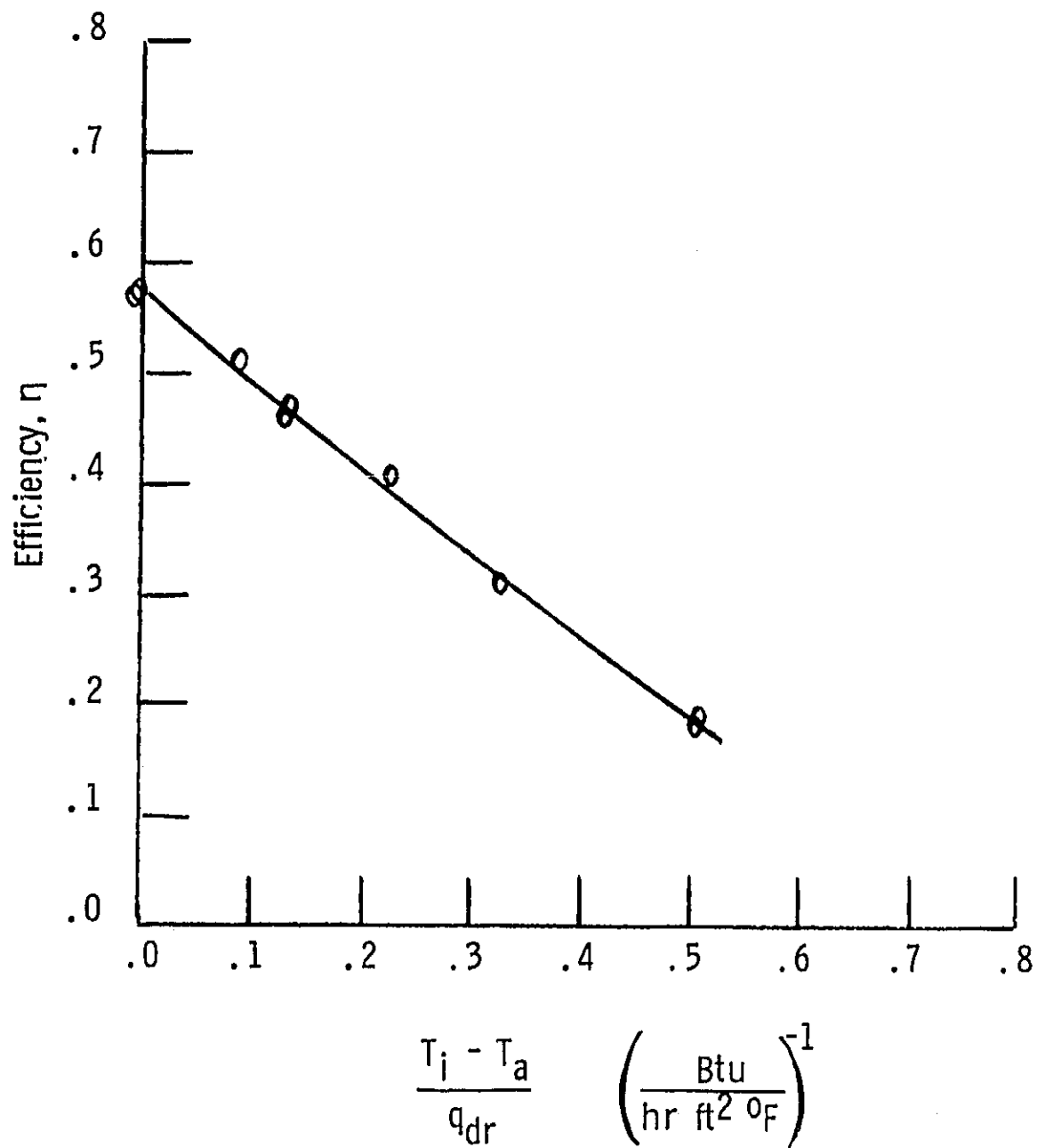
Figure 3.- Collector Performance Correlation
