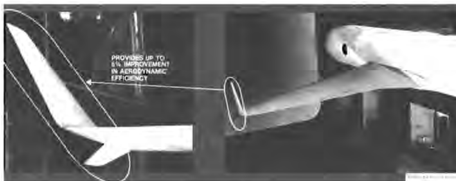
Figure 3 - "Winglet."
